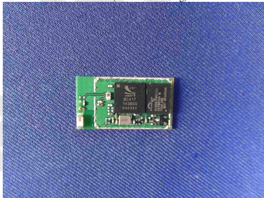
Figure 16 PCB of the EUT-Front View (Without Shielding)
