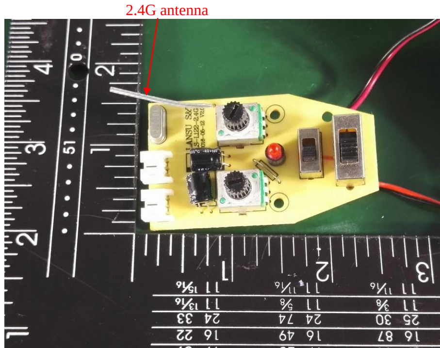
EUT Photo #3 PCB View
