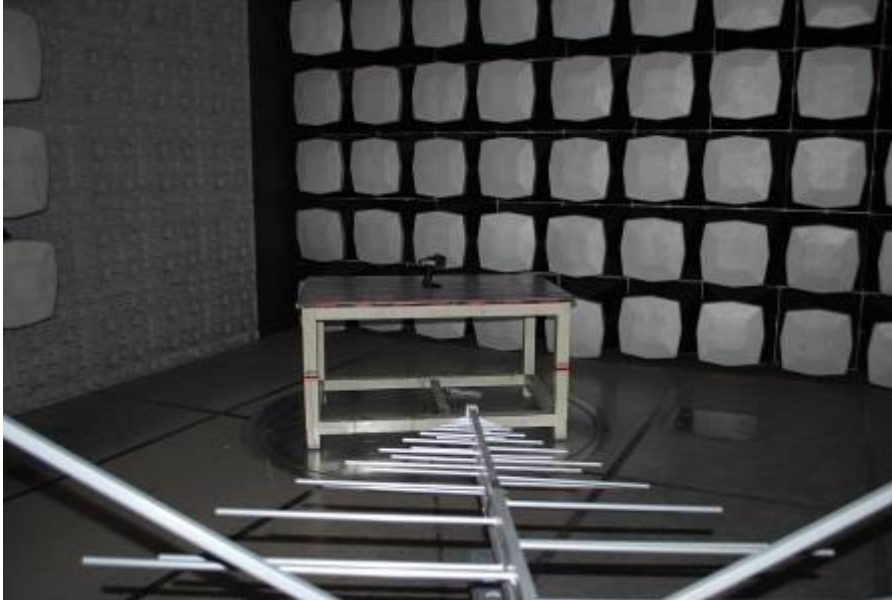
Radiated Emission
