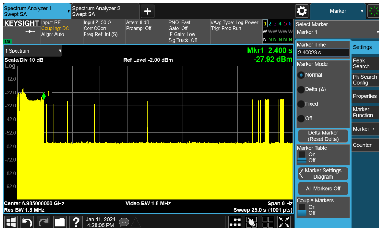
Plot 4: AWGN Signal Detection Details 160MHzBW, 6985-6910MHz
