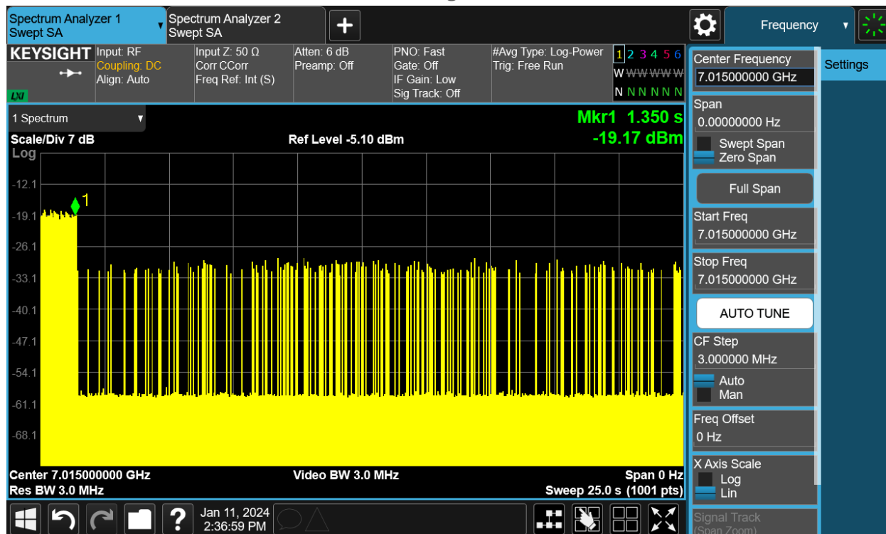
Plot 3: AWGN Signal Detection Details 20MHzBW, 7015MHz
