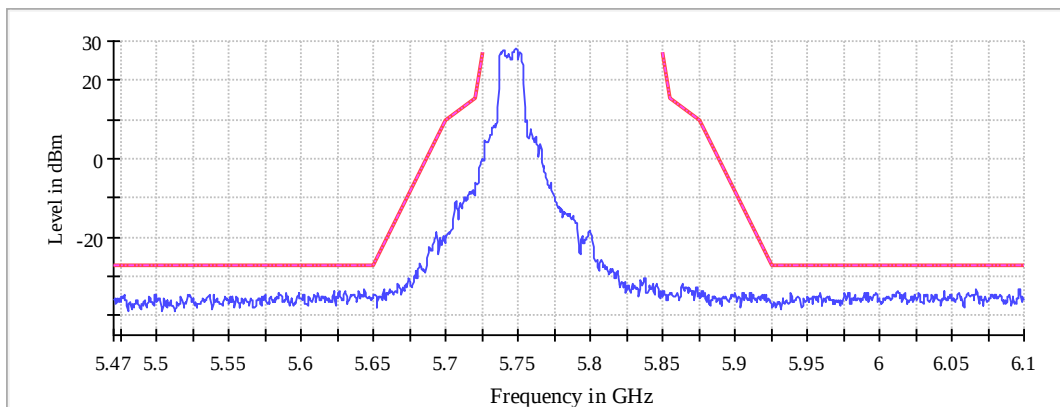
Spurious
