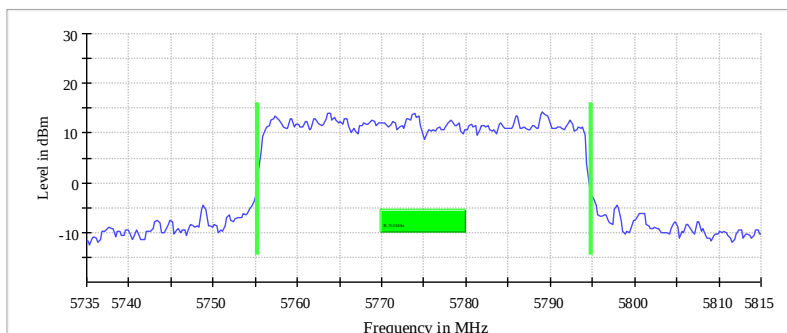
99 % Bandwidth
