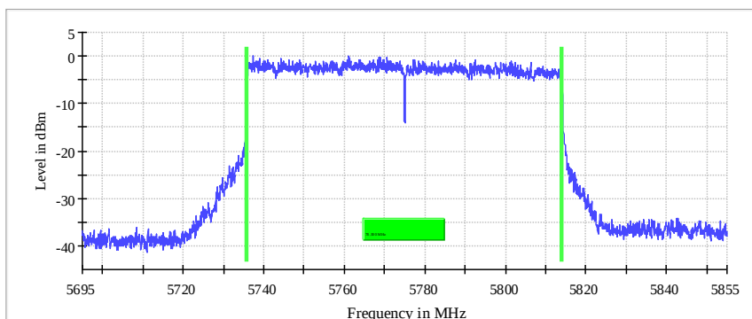
6 dB Bandwidth
