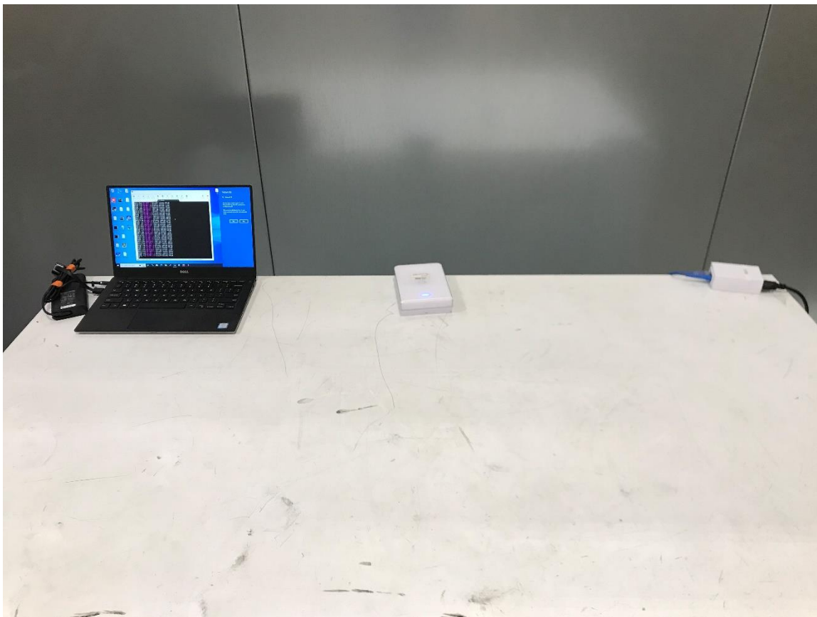
Photograph 6: View Test Set Up Front Conducted Emissions
