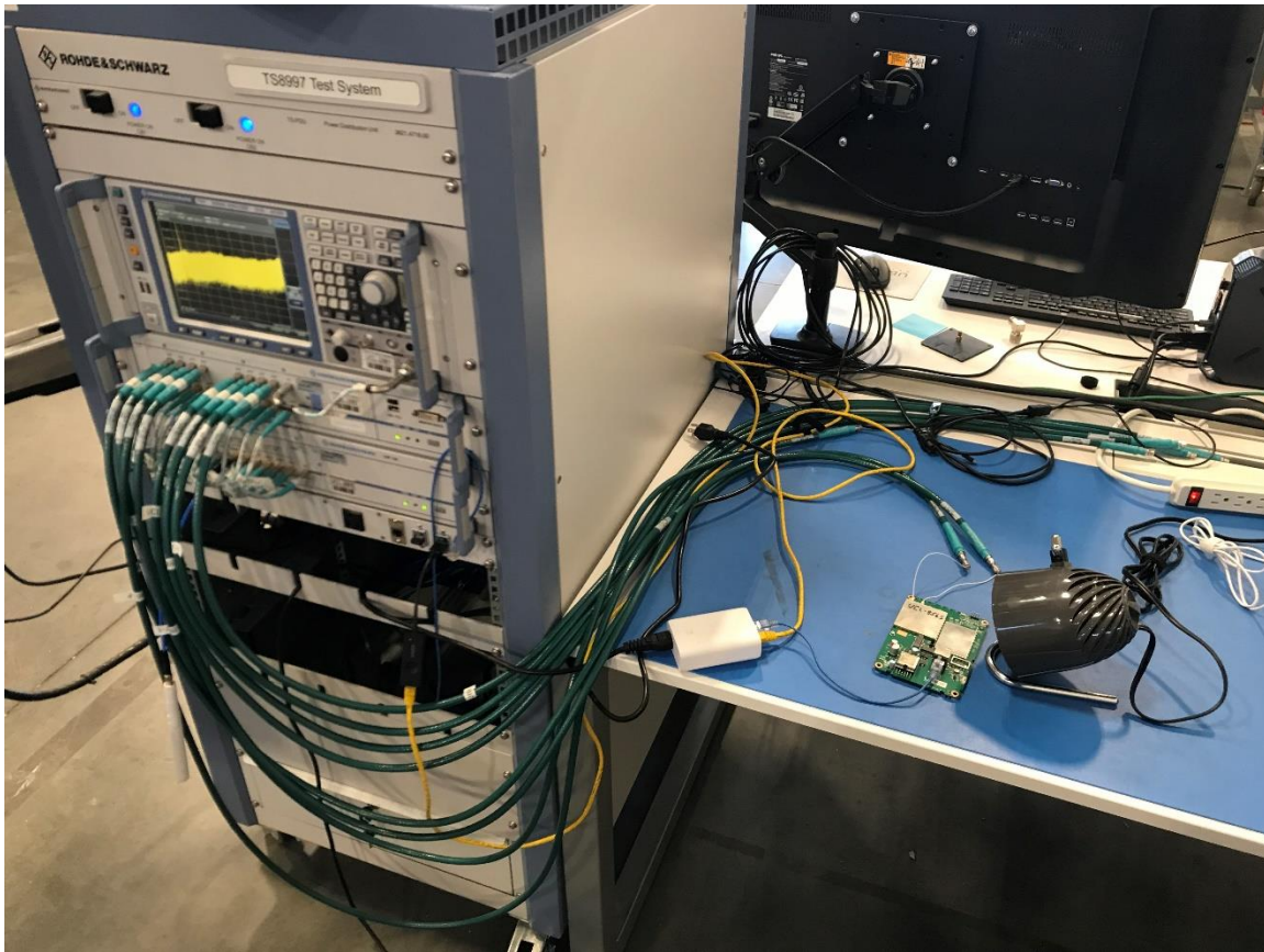
Photograph 4: View Test Set Up RF Conducted
