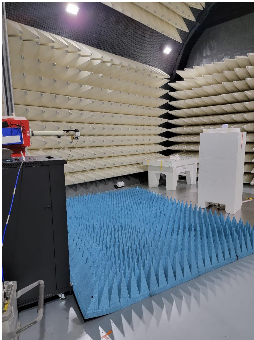
Photograph 3: View Test Set Up Radiated Emissions 17 – 40 GHz
