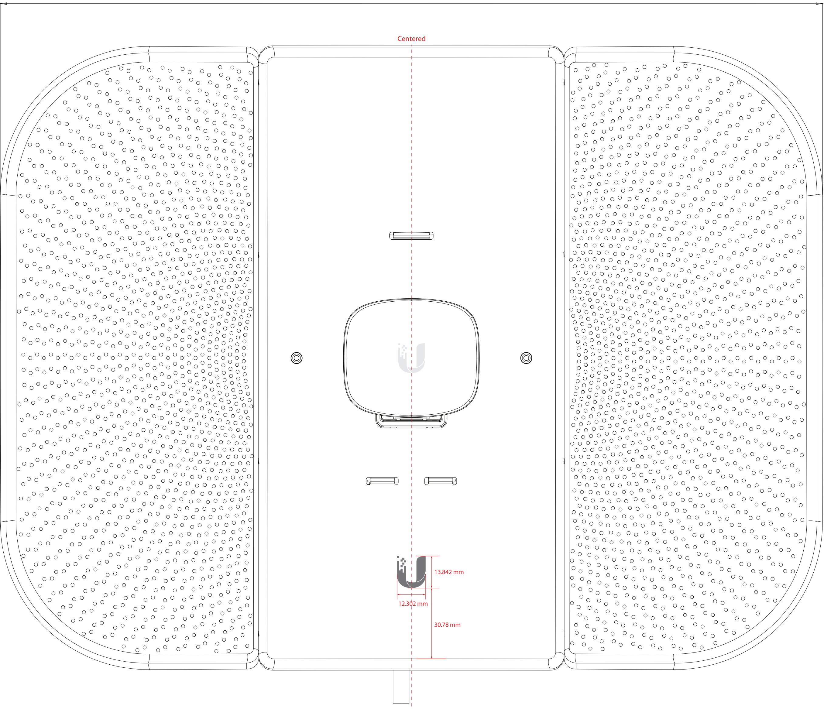
Front View
