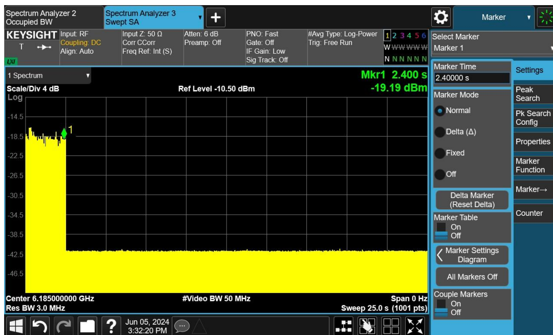
Plot 6: AWGN Signal Detection Details 160 MHz BW, 6185 – 6260
