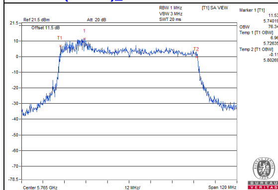
802.11ac (80MHz)_Chain 0 / CH153
