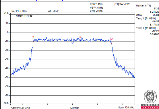
802.11ac (80MHz)_Chain 0 / CH42
