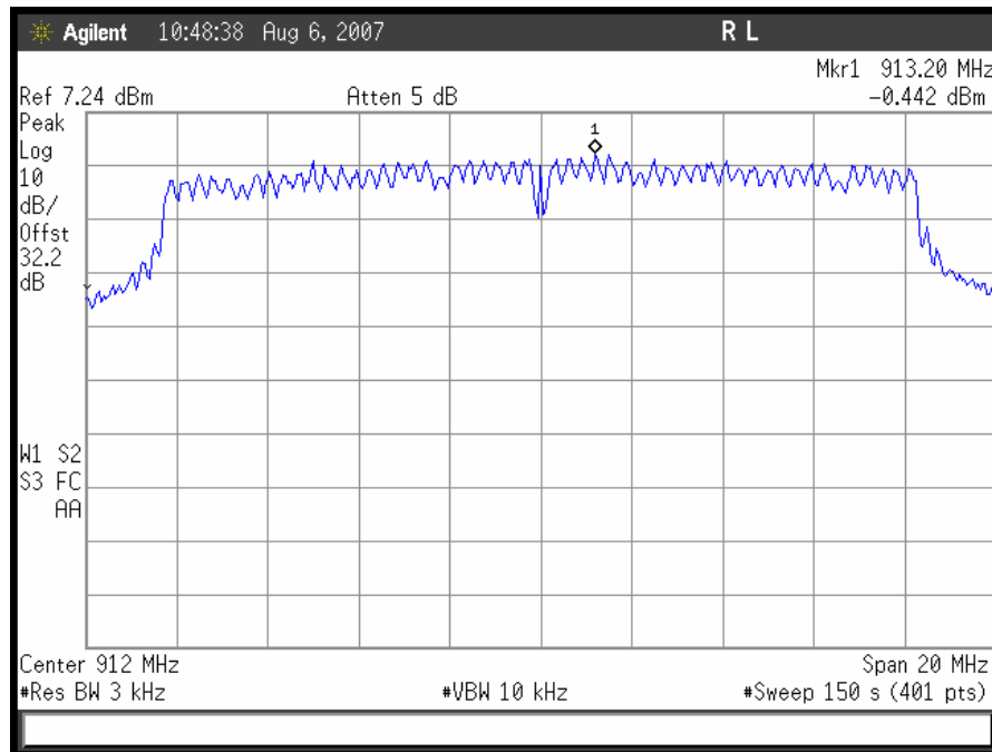
Plot 37. 802.11/g – 912MHz High Ch Peak Power Spectral Density, 20MHz
