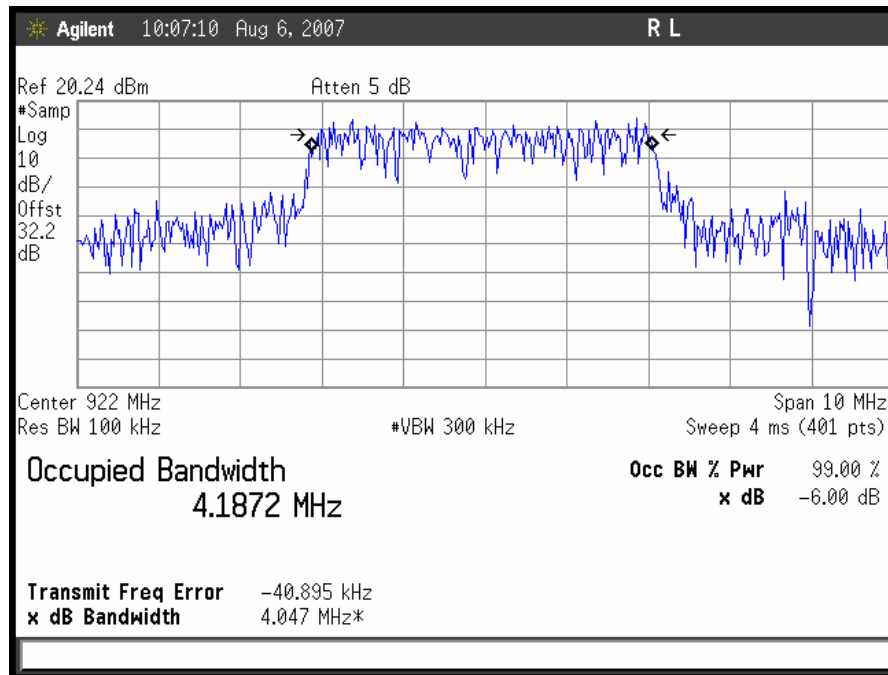
Plot 11. 802.11/g 922MHz Ch Occupied Band Width, 5Mhz
