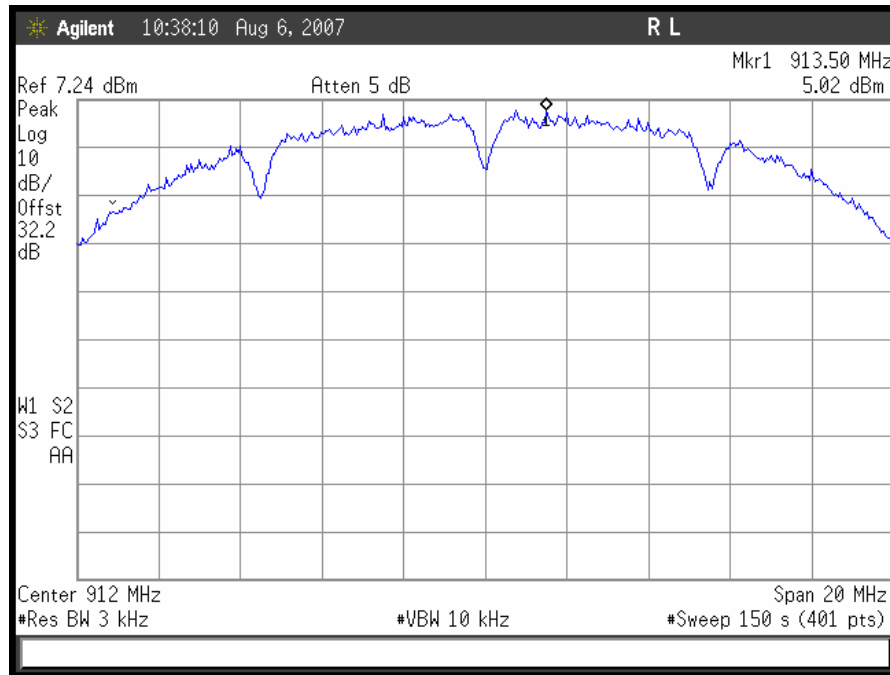
Plot 31. 802.11/b – 912MHz Low Ch Peak Power Spectral Density, 20MHz
