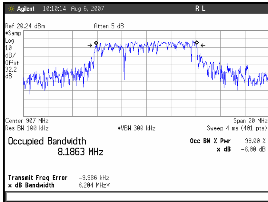
Plot 8. 802.11/g 907MHz Ch Occupied Band Width, 10MHz
