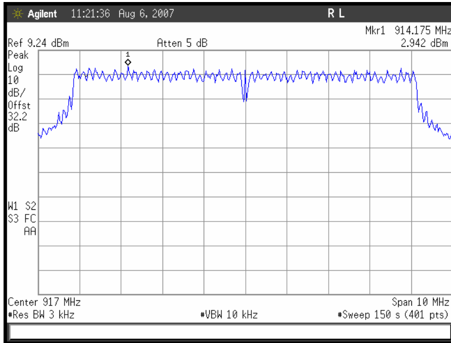
Plot 39. 802.11/g - 917MHz Mid Ch Peak Power Spectral Density, 10MHz
