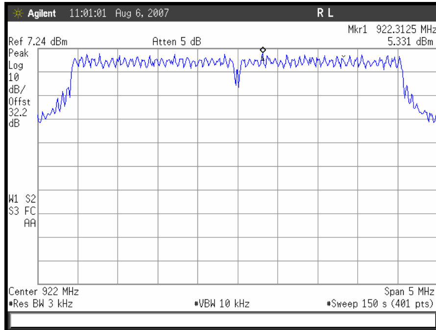
Plot 41. 802.11/g – 922MHz Low Ch Peak Power Spectral Density, 5MHz
