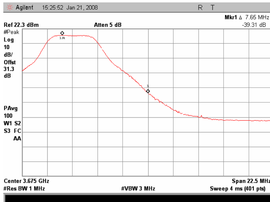
Plot 45. Upper Band Edge 5MHz High Channel
