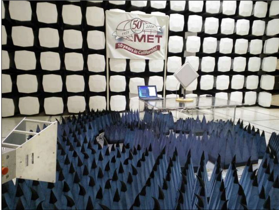
Photograph 5. Radiated Emissions, Test Setup, 1 GHz – 10 GHz
