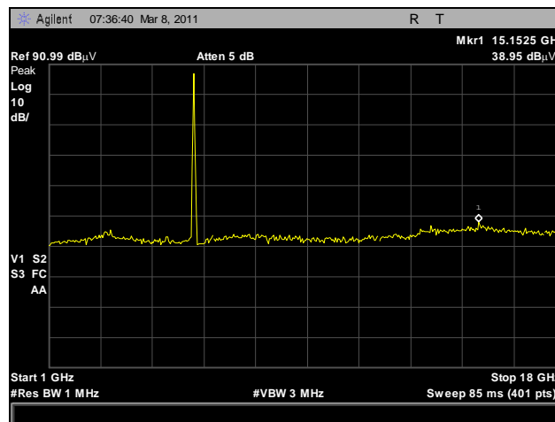
Plot 17. Radiated Spurious Emissions, Low Channel, 1 GHz – 18 GHz
