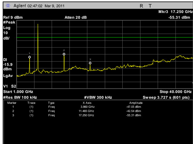
Plot 23. Conducted Spurious Emissions, Low Channel, 1 GHz – 40 GHz
