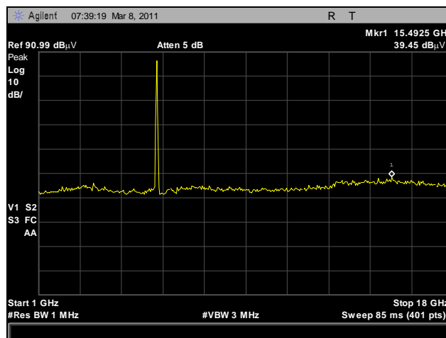
Plot 21. Radiated Spurious Emissions, High Channel, 1 GHz – 18 GHz
