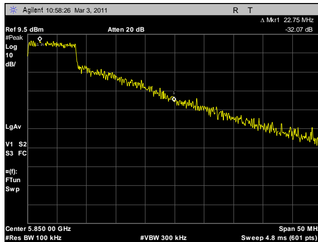
Plot 29. Conducted Band Edge, High Channel
