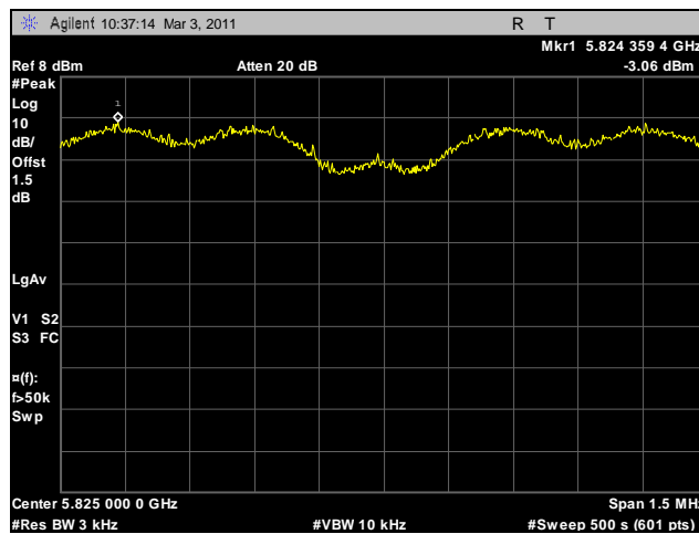
Plot 32. Peak Spectral Density, High Channel
