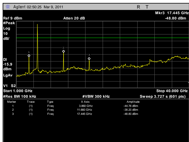
Plot 27. Conducted Spurious Emissions, High Channel, 1 GHz – 40 GHz
