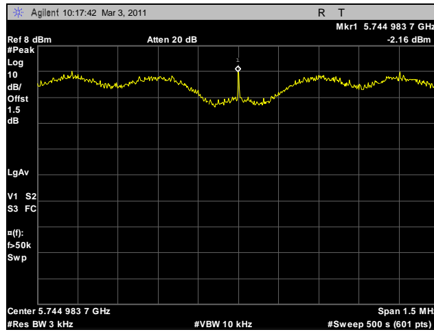
Plot 30. Peak Spectral Density, Low Channel
