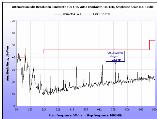
Plot 18. Radiated Spurious Emissions, Mid Channel, 30 MHz – 1 GHz
