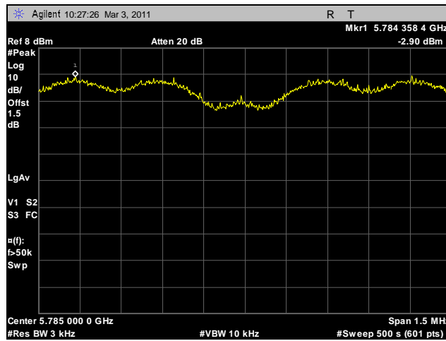
Plot 31. Peak Spectral Density, Mid Channel
