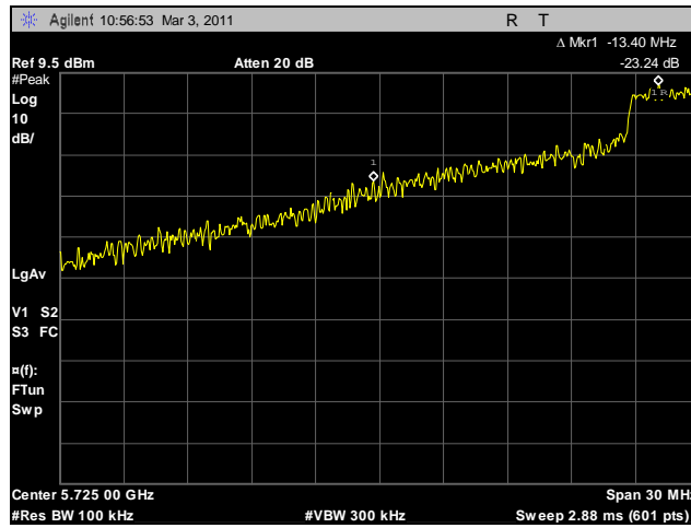
Plot 28. Conducted Band Edge, Low Channel
