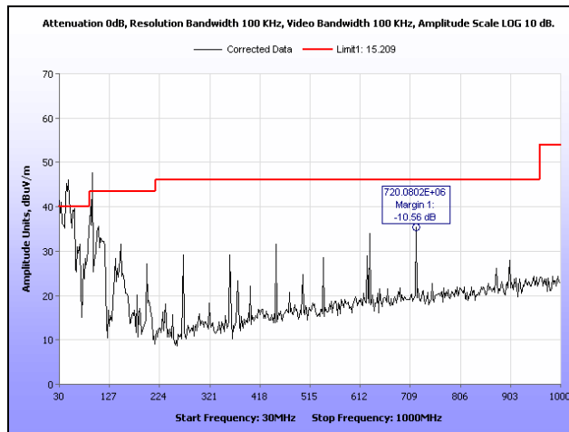
Plot 20. Radiated Spurious Emissions, High Channel, 30 MHz – 1 GHz
