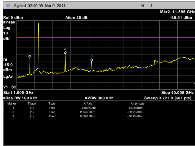
Plot 25. Conducted Spurious Emissions, Mid Channel, 1 GHz – 40 GHz
