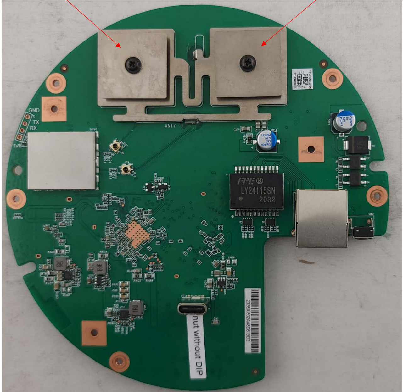
Photograph 2: Internal View of Main PCB Top
