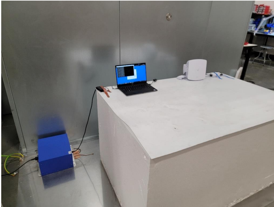
Photograph 5: Front View Test Set Up AC Mains Conducted Emissions
