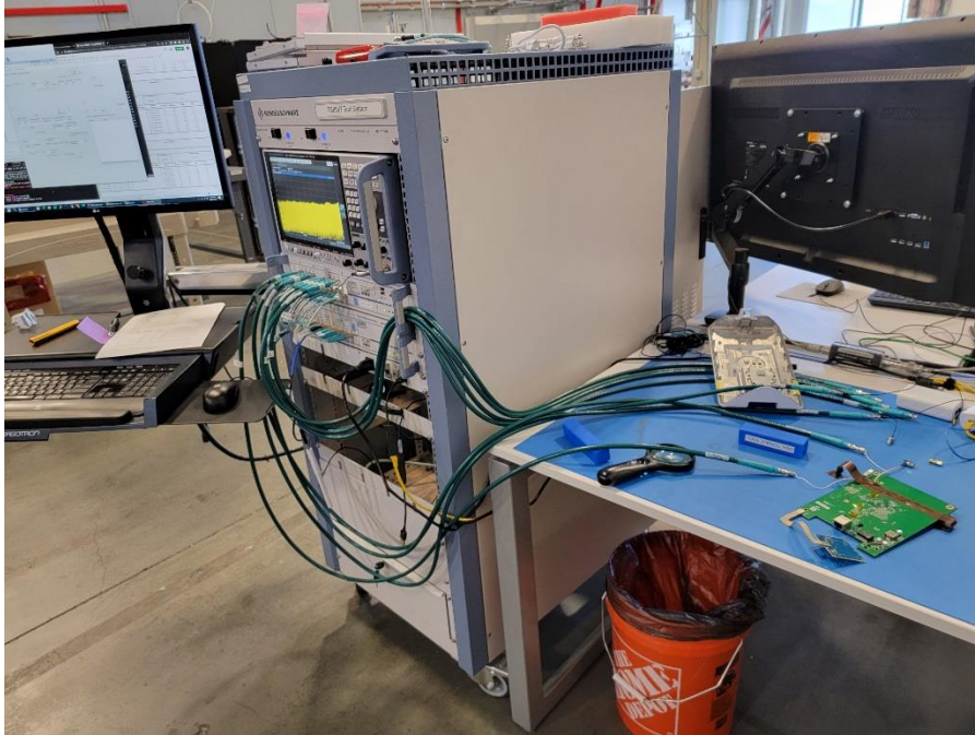
Photograph 5: View Test Set Up RF Conducted
