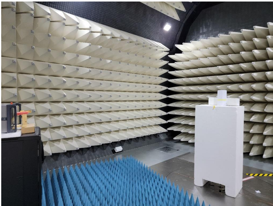
Photograph 4: View Test Set Up Radiated Emissions 40 – 220 GHz
