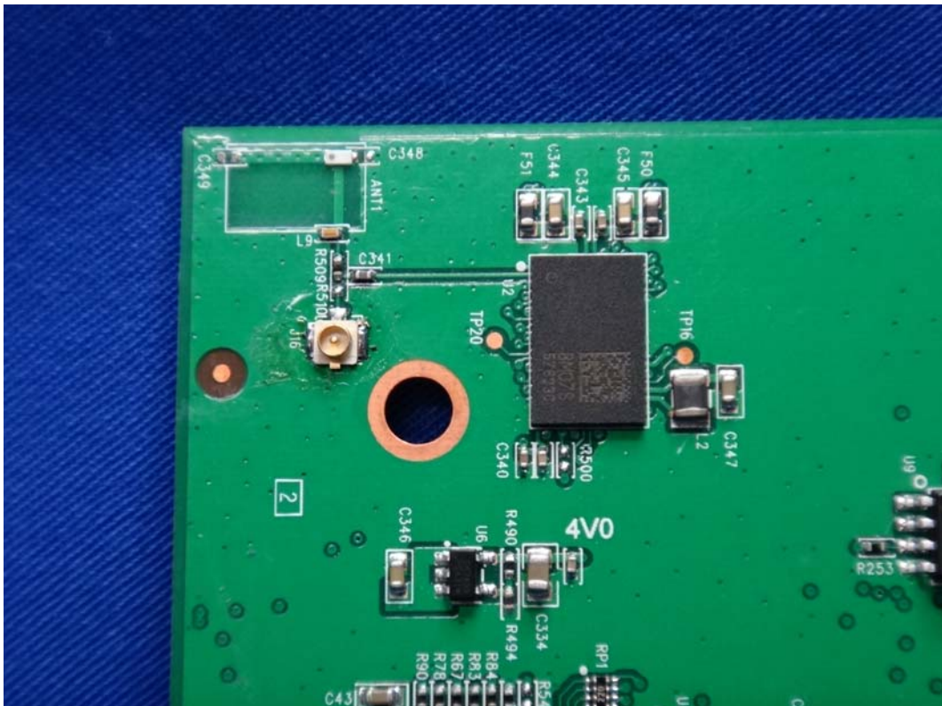
(22) EUT Photo-RF Chip & Chip Antenna
