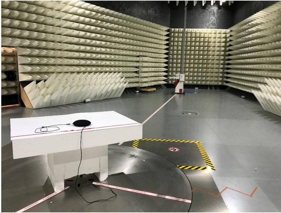
Photograph 1: Test Set Up Radiated Emissions 30 – 1000 MHz
