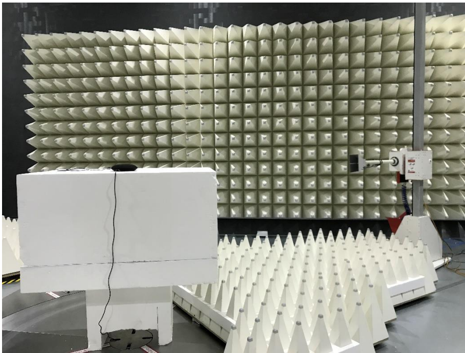
Photograph 2: Test Set Up Radiated Emissions 1 – 40 GHz
