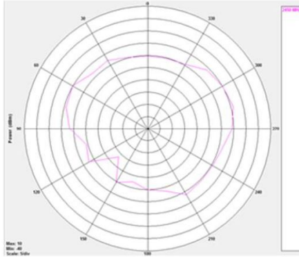
X-Z Plane (E-total)
