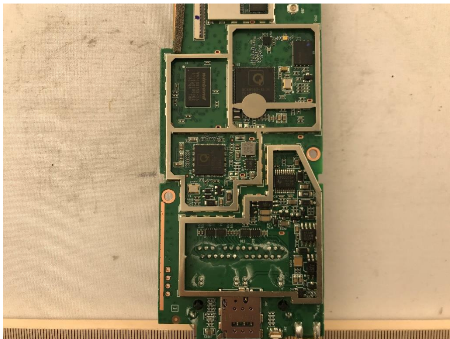
Photograph 8: Close-Up Bottom of Side B
