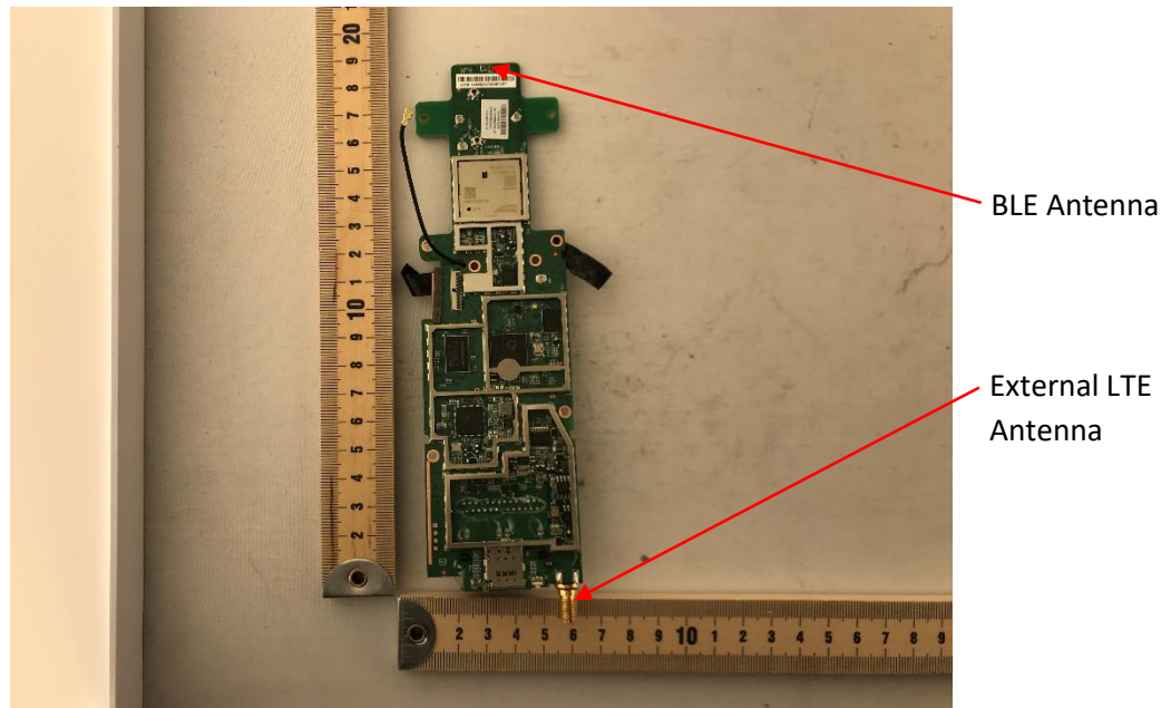
Photograph 1: View of Circuit Board Inside/Outside Housing
