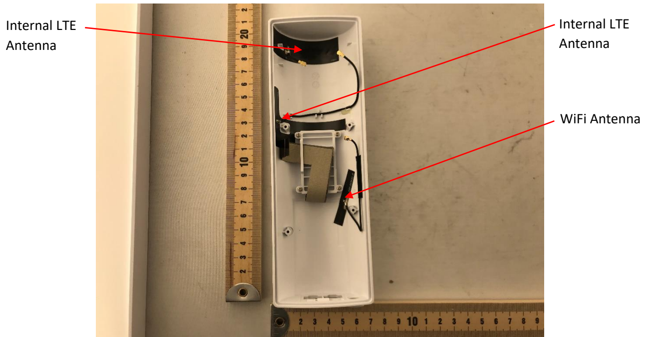
Photograph 4: Housing View of Circuit Board
