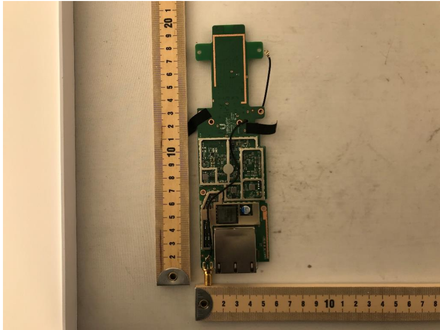
Photograph 3: Bottom View of Circuit Board
