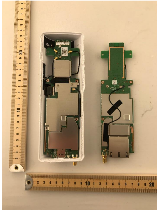
Photograph 1: View of Circuit Board Inside/Outside Housing
