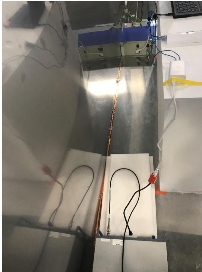
Photograph 5: Back View Test Set Up Conducted Emissions
