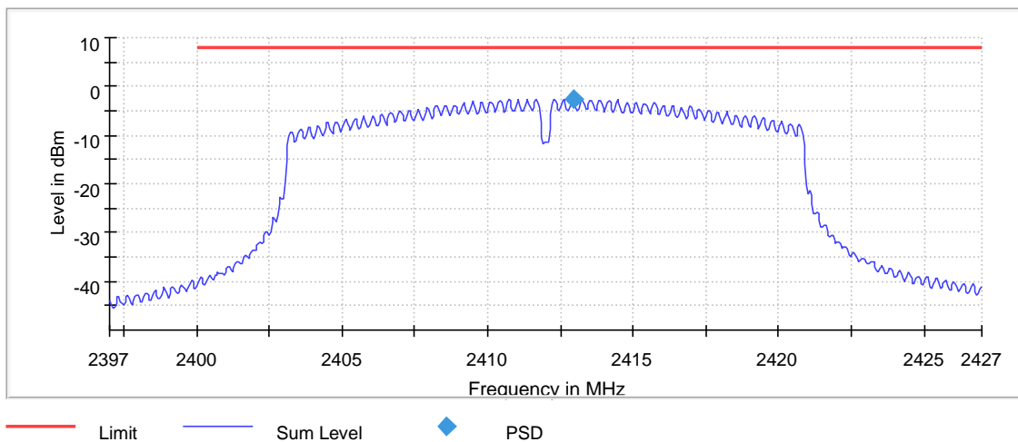
Graph 37: 2412 (N-Mode - 20MHz) Lowest Channel 3 kHz PSD Plot
