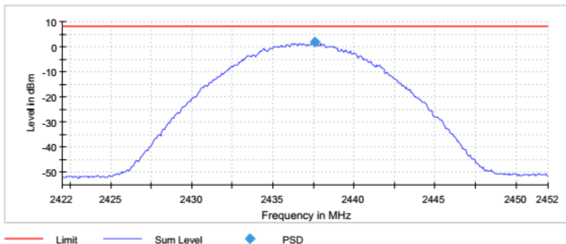
Graph 12: 2437 (B-Mode) Middle Channel 3 kHz PSD Plot
