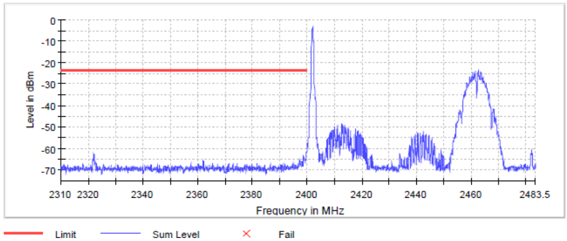
Graph 63: 2402 (BLE-Mode) Lower Band Edge Plot
