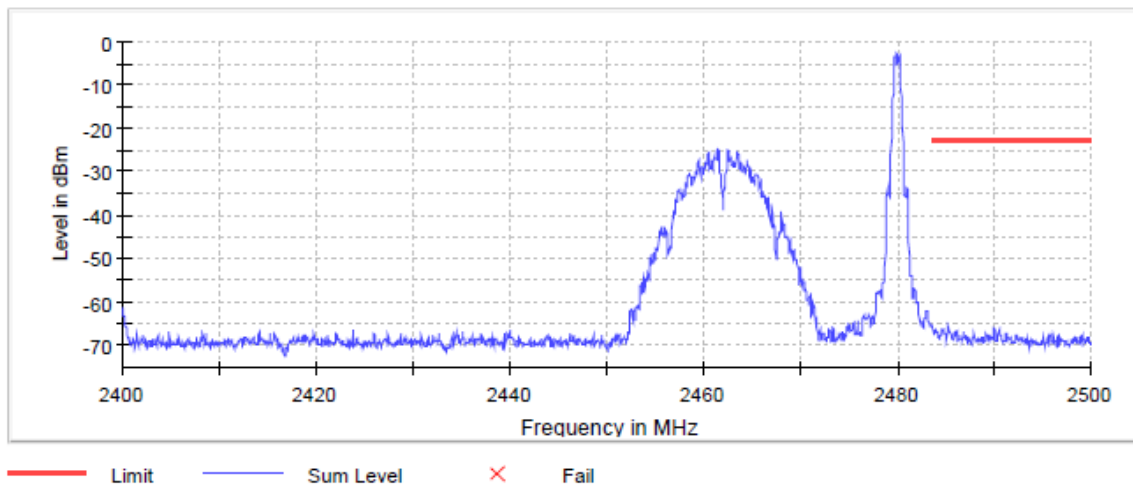
Graph 64: 2480 (BLE-Mode) Upper Band Edge Plot
