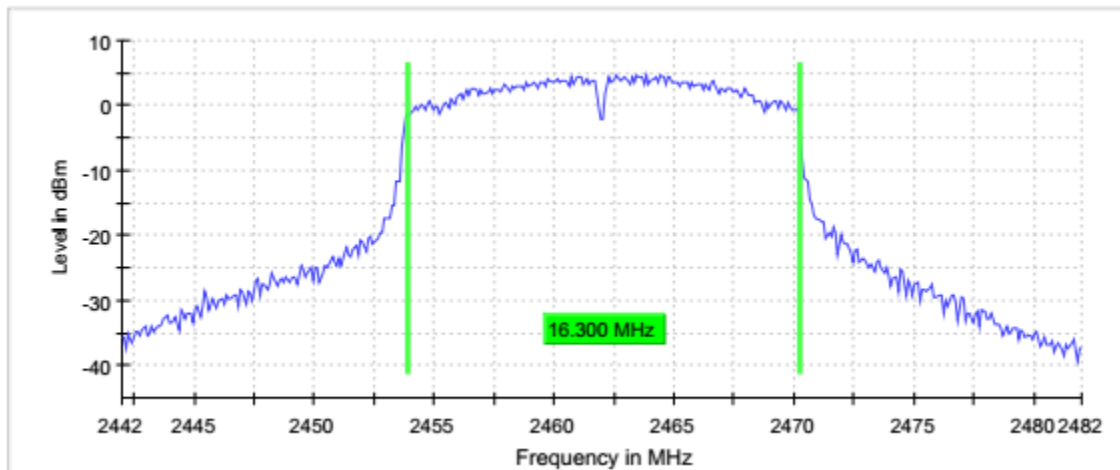
Graph 16: 2462 (G-Mode) 6dB Emissions Bandwidth
