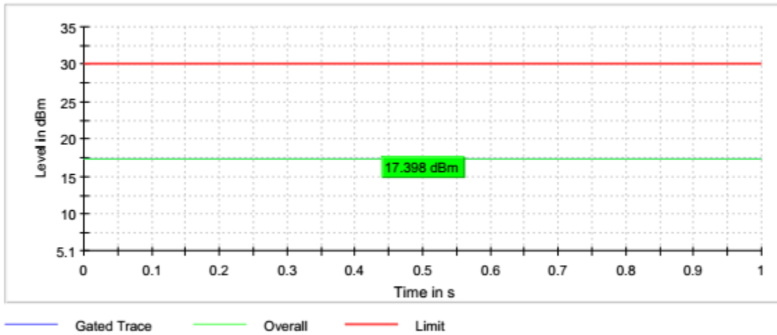
Graph 18: 2437 (G-Mode) Peak Output Power
