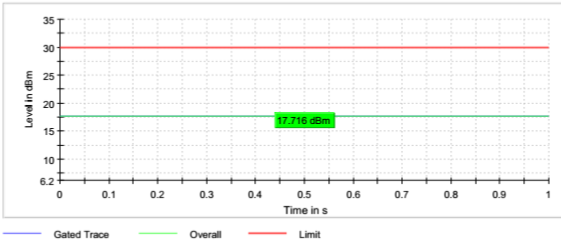
Graph 17: 2412 (G-Mode) Peak Output Power
