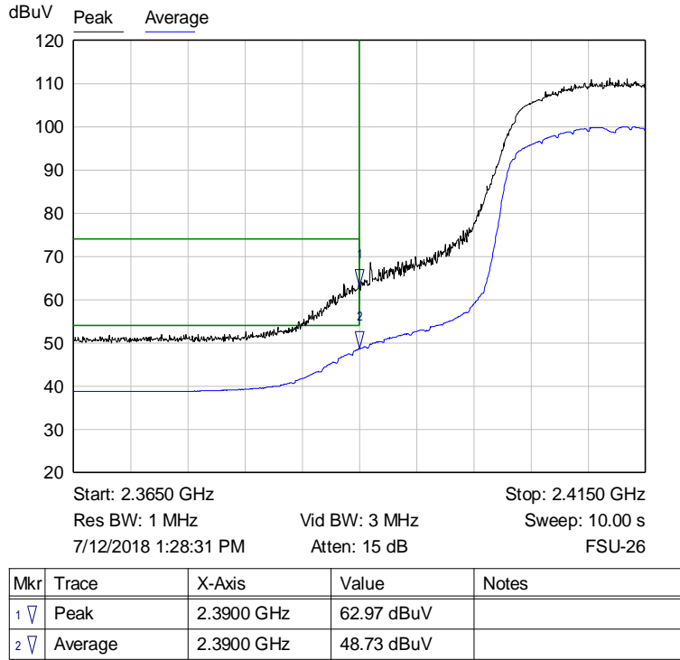
Graph 35: Radiated Lower Band Edge Plot
