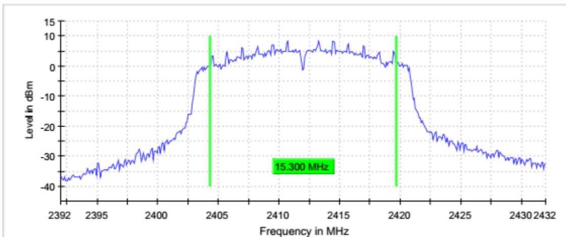
Graph 27: 2412 (N-Mode – 20MHz) 6dB Emissions Bandwidth
