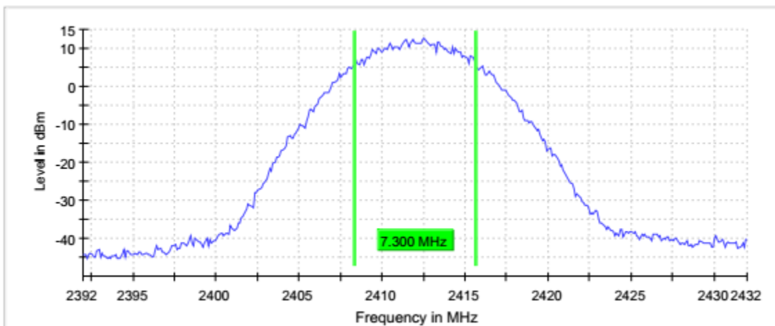
Graph 1: 2412 (B-Mode) 6dB Emissions Bandwidth
