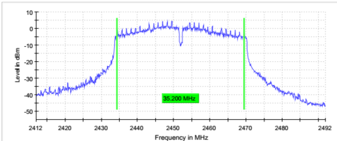
Graph 42: 2452 (N-Mode - 40MHz) 6dB Emissions Bandwidth
