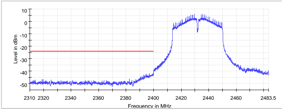
Graph 46: (N-Mode - 40MHz) Lower Band Edge Plot
