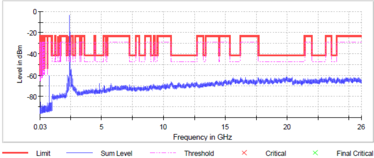
Graph 60: 2402 (BLE-Mode) Spurious Emissions Plot
