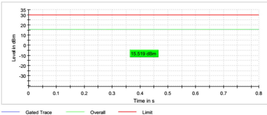
Graph 45: 2452 (N-Mode – 40MHz) Maximum Average Output Power
