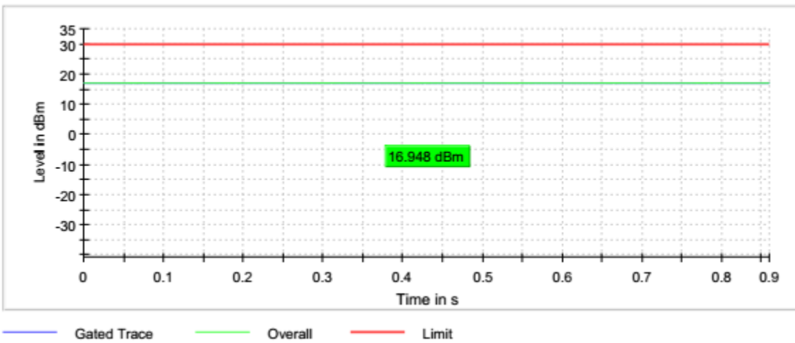
Graph 44: 2437 (N-Mode – 40MHz) Maximum Average Output Power
