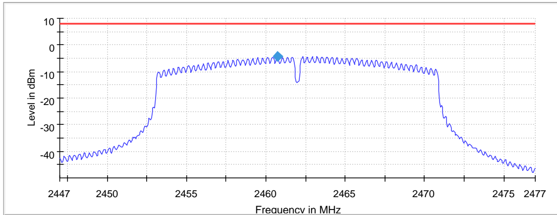
Graph 39: 2462 (N-Mode – 20MHz) Highest Channel Output 3 kHz PSD Plot
