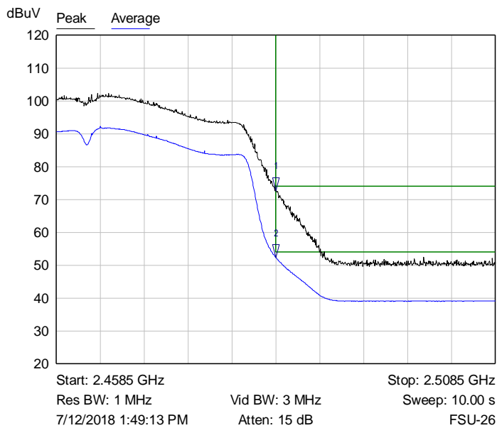
Graph 49: Radiated Band Edge Plot (Channel 9)
