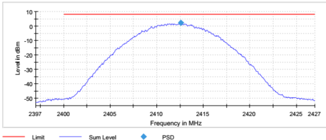
Graph 11: 2412 (B-Mode) Lowest Channel 3 kHz PSD Plot
