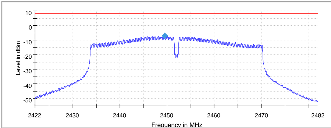
Graph 53: 2452 (N-Mode – 40MHz) Highest Channel Output 3 kHz PSD Plot
