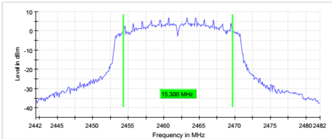
Graph 29: 2462 (N-Mode – 20MHz) 6dB Emissions Bandwidth
