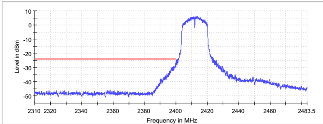
Graph 20: (G-Mode) Lower Band Edge Plot
