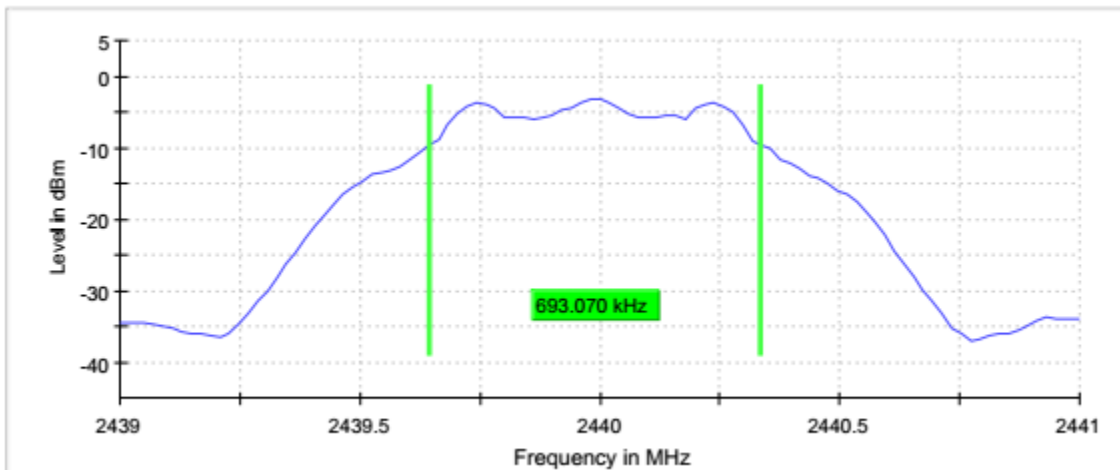
Graph 55: 2440 (BLE-Mode) Middle Channel Bandwidth
