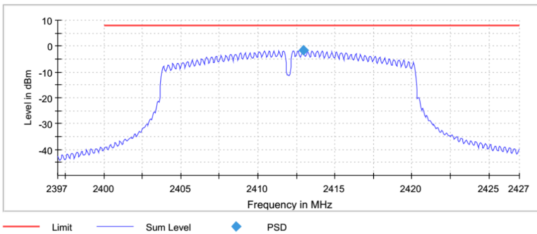
Graph 24: 2412 (G-Mode) Lowest Channel 3 kHz PSD Plot
