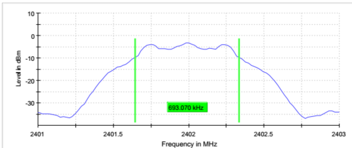
Graph 54: 2402 (BLE-Mode) Lowest Channel Bandwidth
