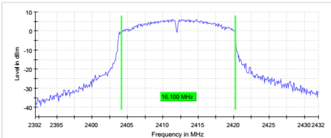
Graph 14: 2412 (G-Mode) 6dB Emissions Bandwidth
