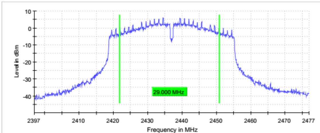
Graph 41: 2437 (N-Mode - 40MHz) 6dB Emissions Bandwidth
