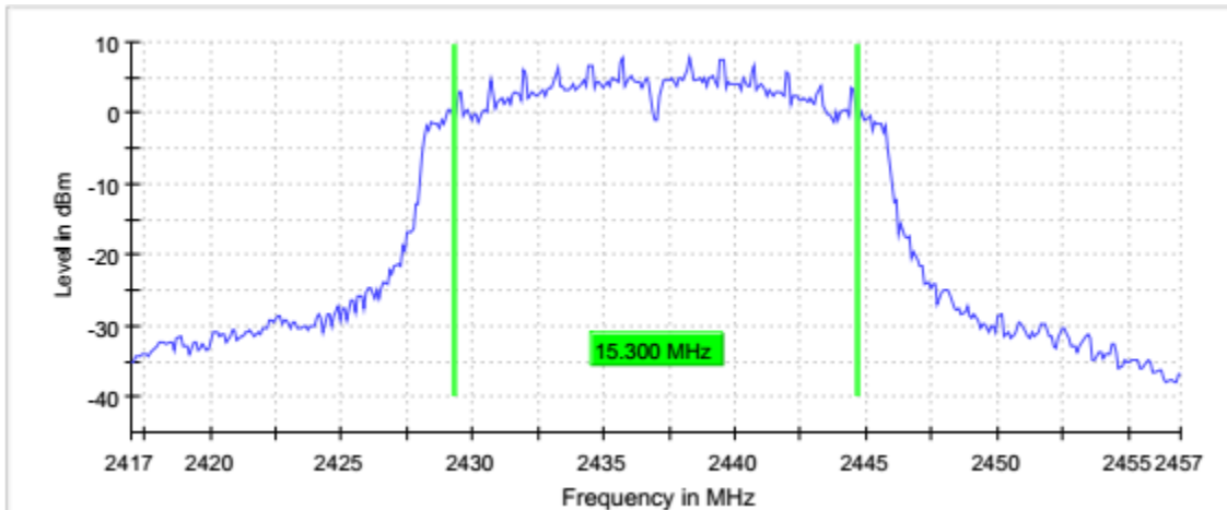
Graph 28: 2437 (N-Mode – 20MHz) 6dB Emissions Bandwidth
