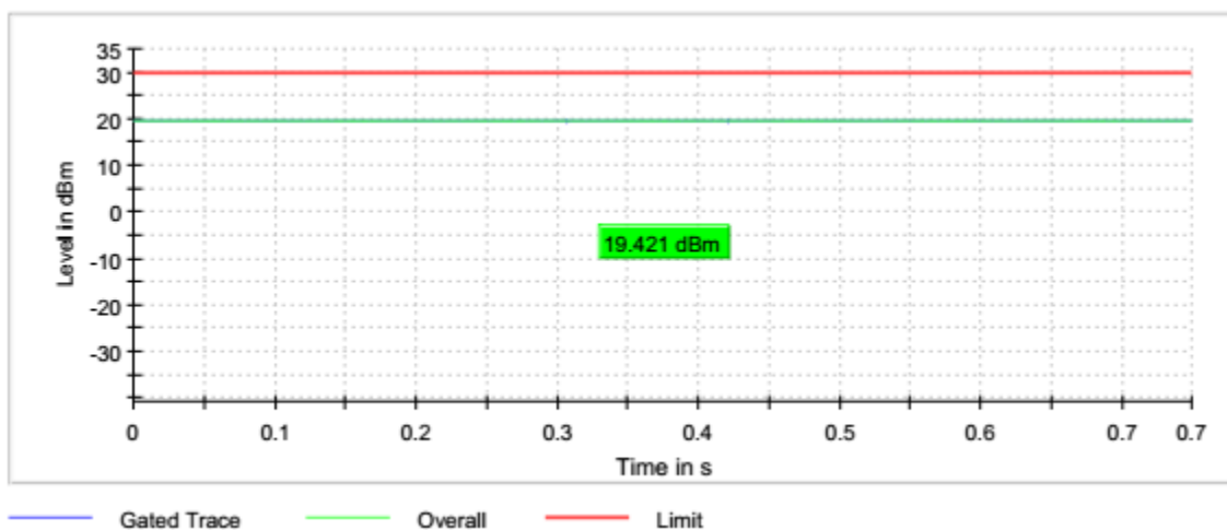
Graph 4: 2412 (B-Mode - 20MHz) Maximum Average Output Power
