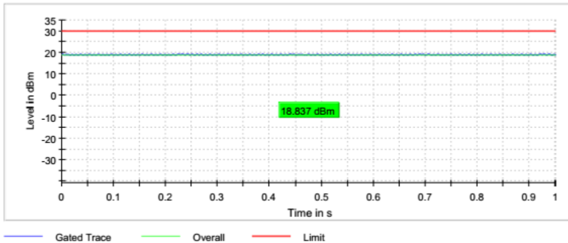
Graph 5: 2437 (B-Mode – 20MHz) Maximum Average Output Power
