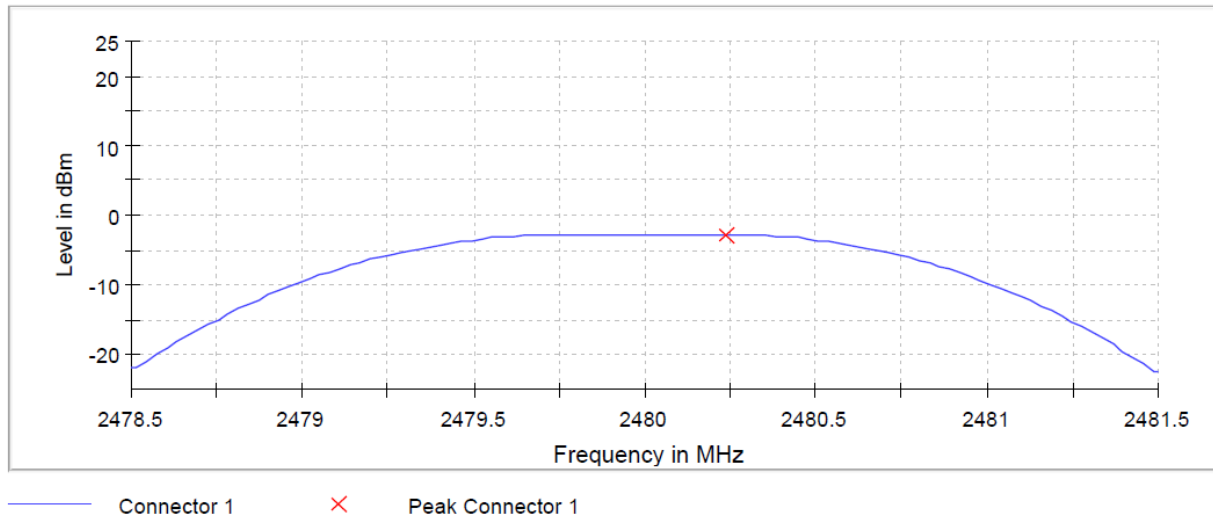
Graph 59: 2480 (BLE-Mode) Highest Channel Output Power Plot
