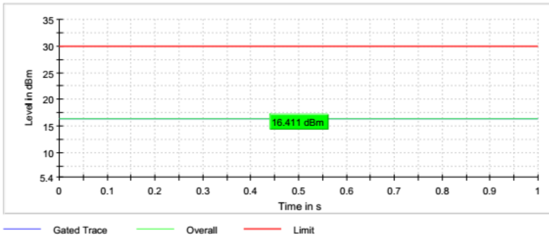
Graph 19: 2462 (G-Mode) Peak Output Power
