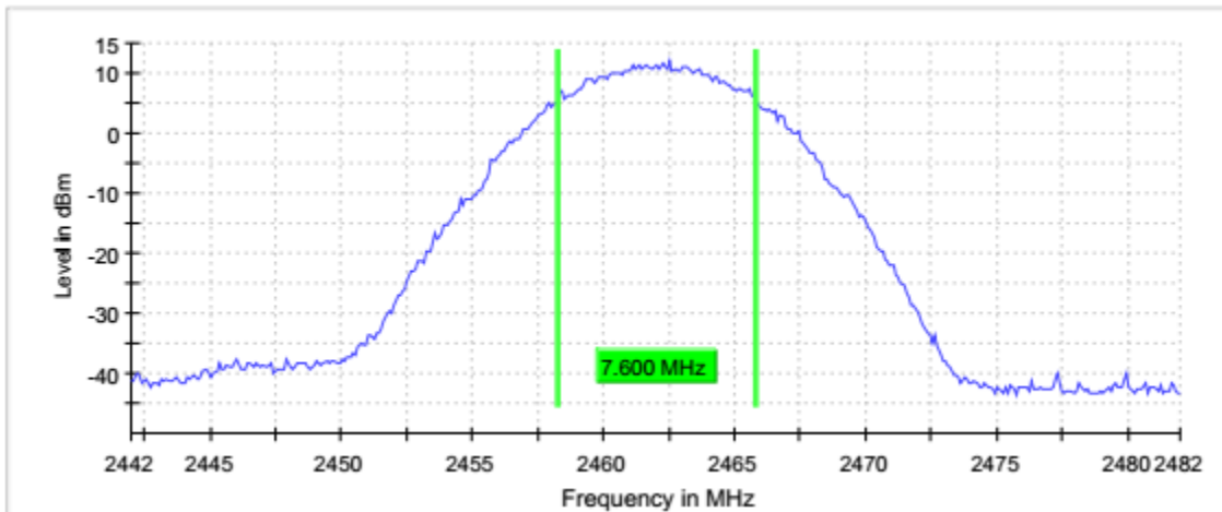
Graph 3: 2462 (B-Mode) 6dB Emissions Bandwidth
