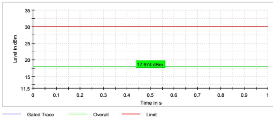
Graph 6: 2462 (B-Mode) Maximum Average Output Power
