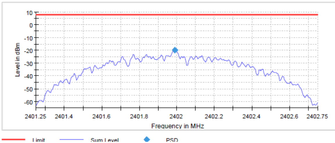
Graph 67: 2402 (BLE-Mode) Lowest Channel 3 kHz PSD Plot
