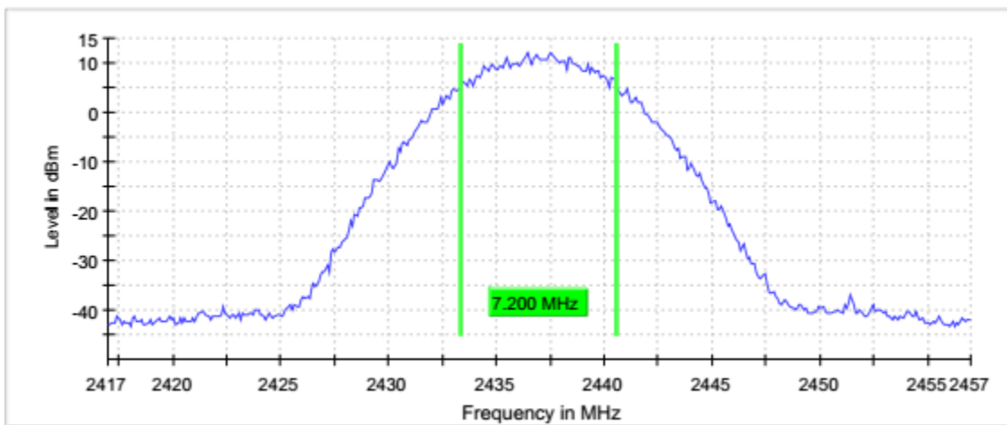
Graph 2: 2437 (B-Mode) 6dB Emissions Bandwidth
