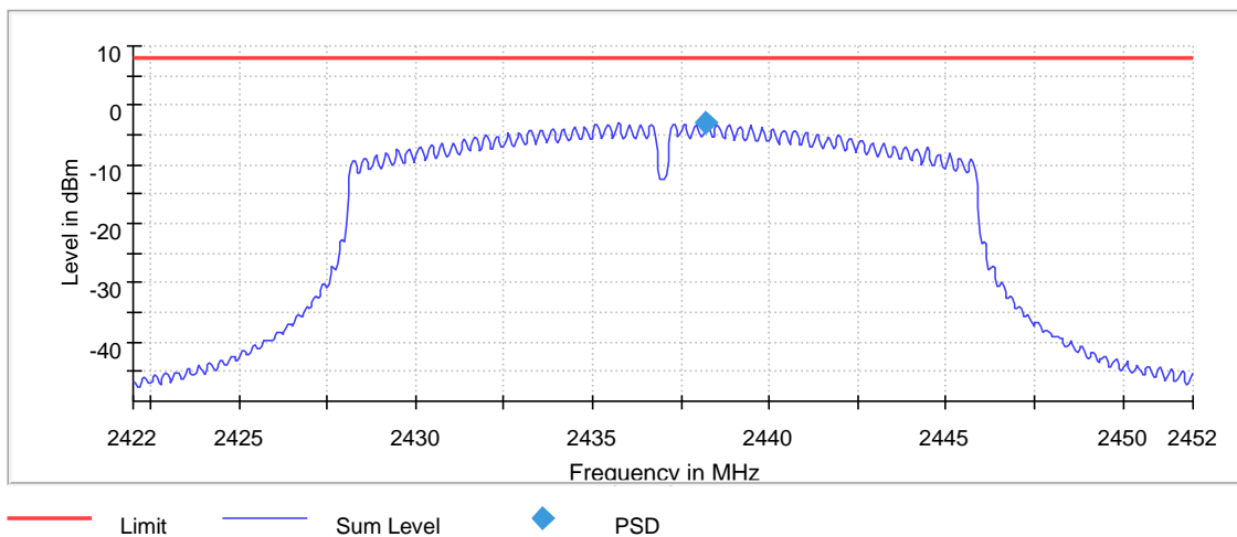
Graph 38: 2437 (N-Mode - 20MHz) Middle Channel 3 kHz PSD Plot
