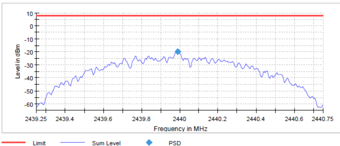
Graph 68: 2440 (BLE-Mode) Middle Channel 3 kHz PSD Plot
