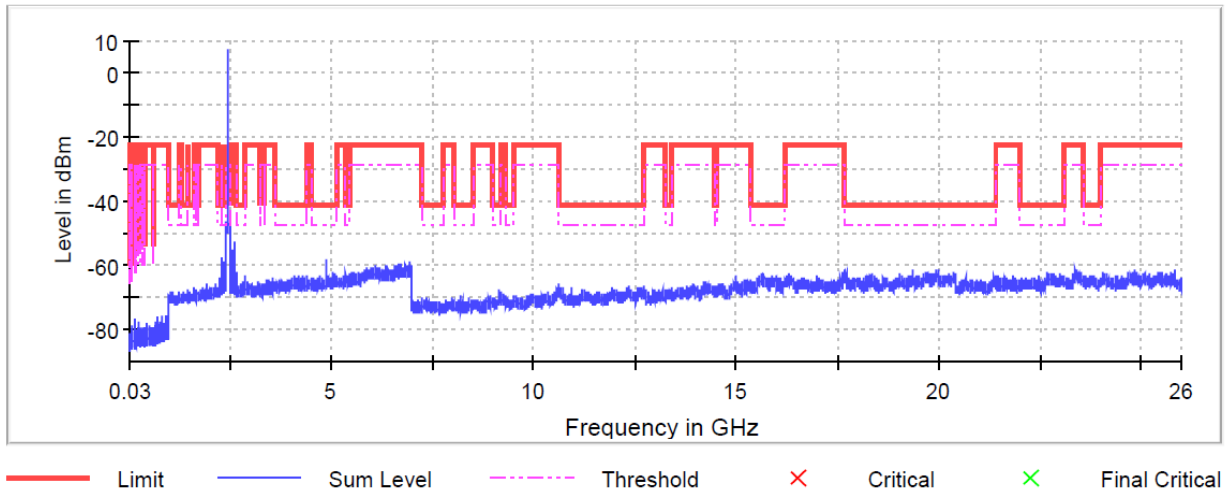
Graph 61: 2440 (BLE-Mode) Spurious Emissions Plot
