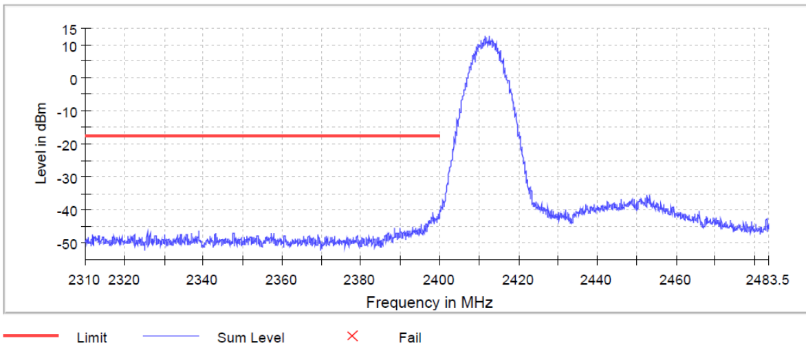
Graph 7: (B-Mode) Lower Band Edge Plot
