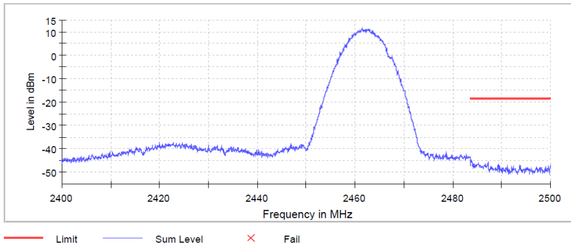
Graph 8: (B-Mode) Upper Band Edge Plot
