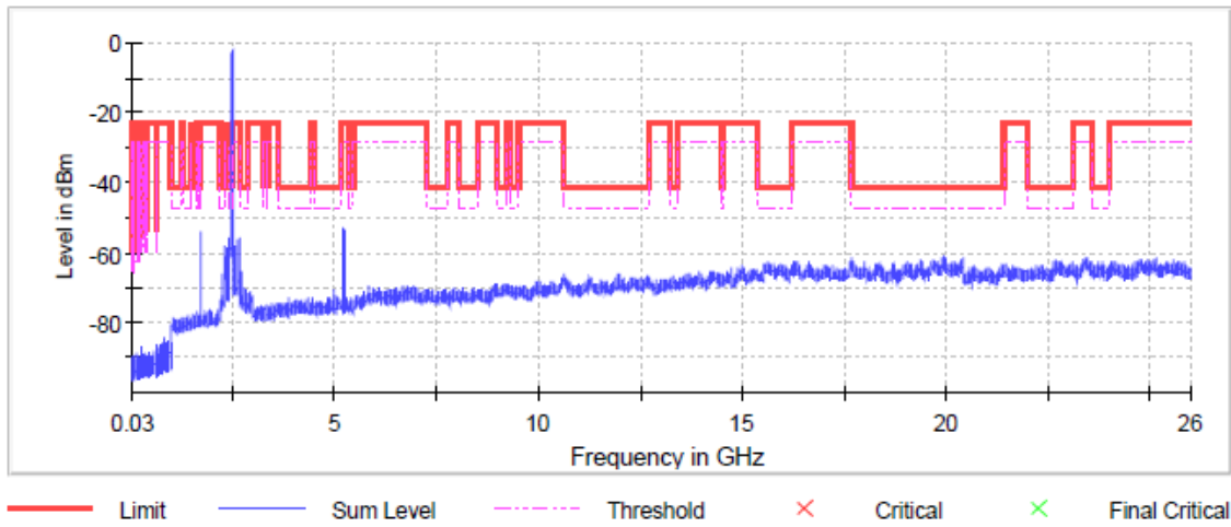
Graph 62: 2480 (BLE-Mode) Spurious Emissions Plot
