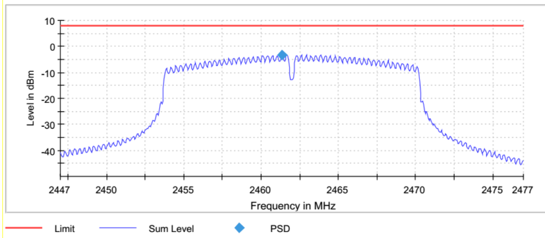
Graph 26: 2462 (G-Mode) Highest Channel Output 3 kHz PSD Plot
