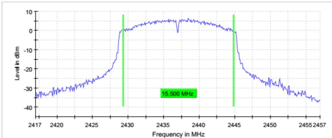
Graph 15: 2437 (G-Mode) 6dB Emissions Bandwidth
