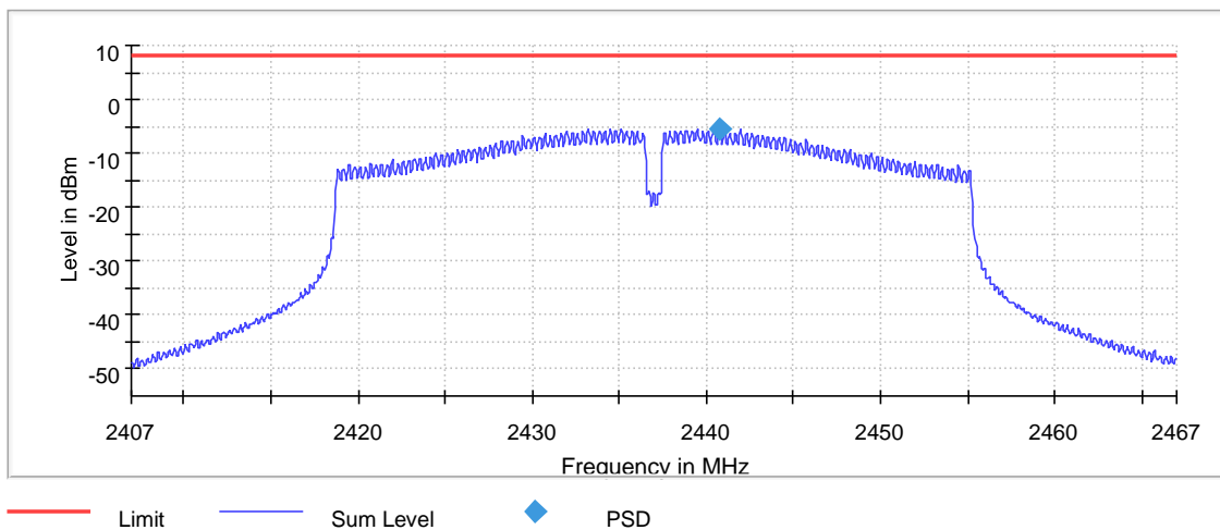
Graph 52: 2437 (N-Mode - 40MHz) Middle Channel 3 kHz PSD Plot
