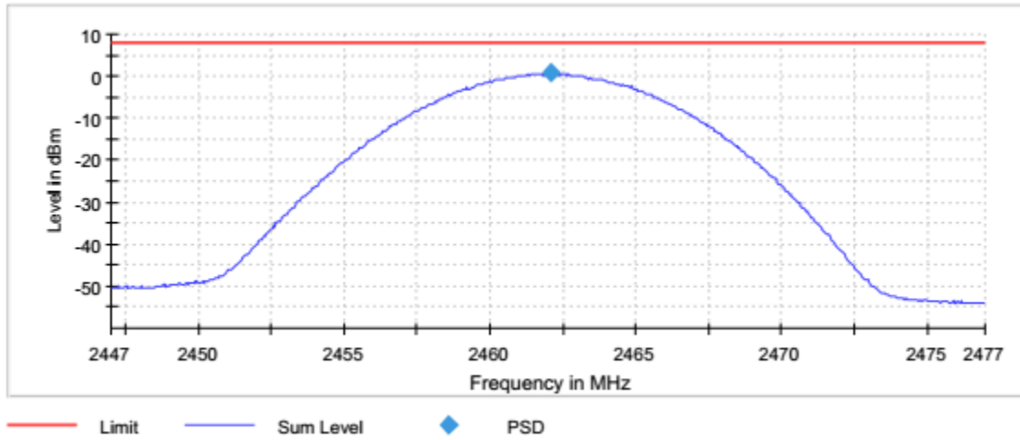
Graph 13: 2462 (B-Mode) Highest Channel Output 3 kHz PSD Plot
