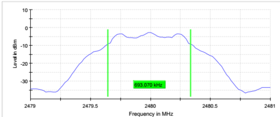
Graph 56: 2480 (BLE-Mode) Highest Channel Bandwidth
