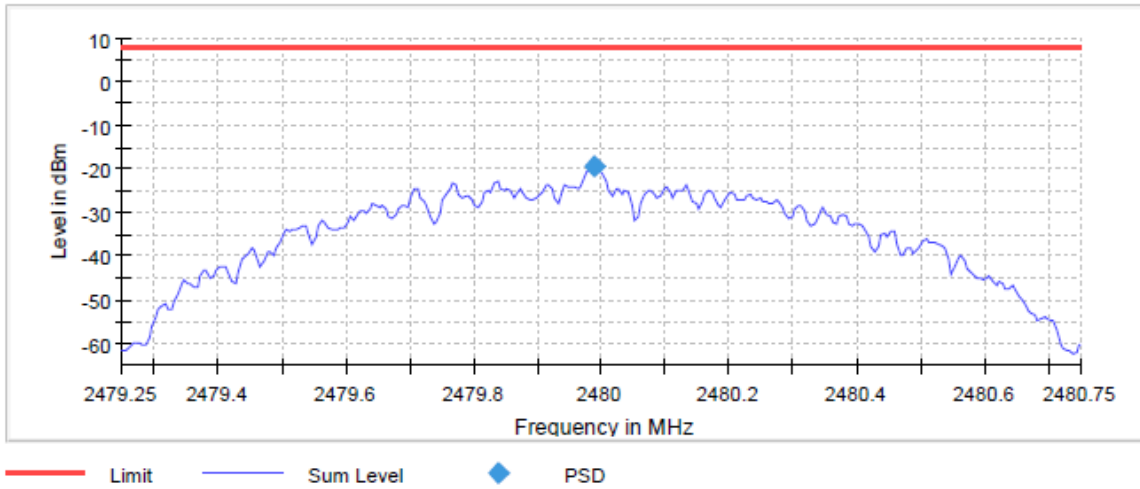
Graph 69: 2480 (BLE-Mode) Highest Channel Output 3 kHz PSD Plot
