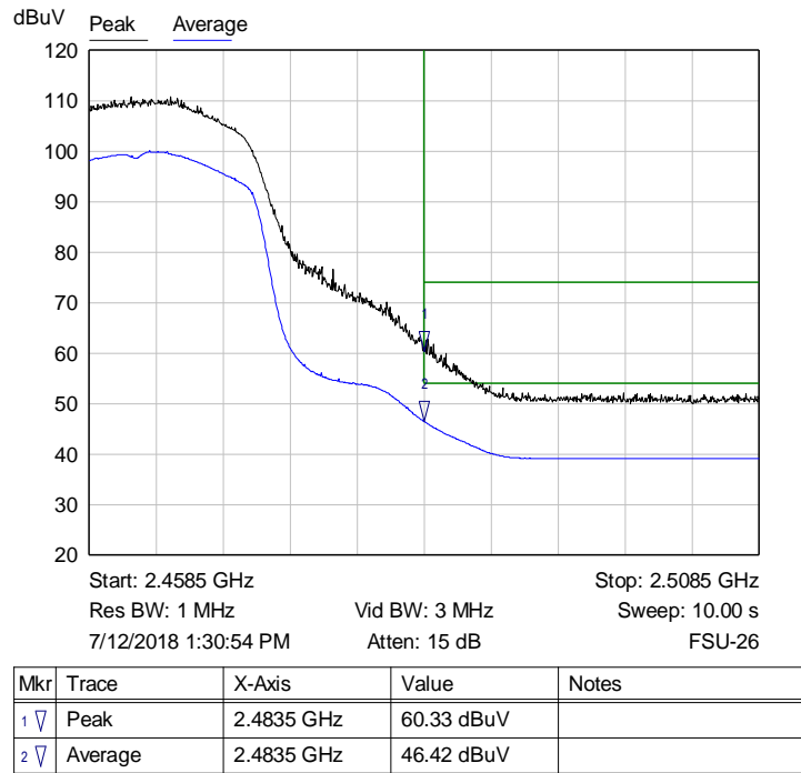
Graph 36: Radiated Upper Band Edge Plot
