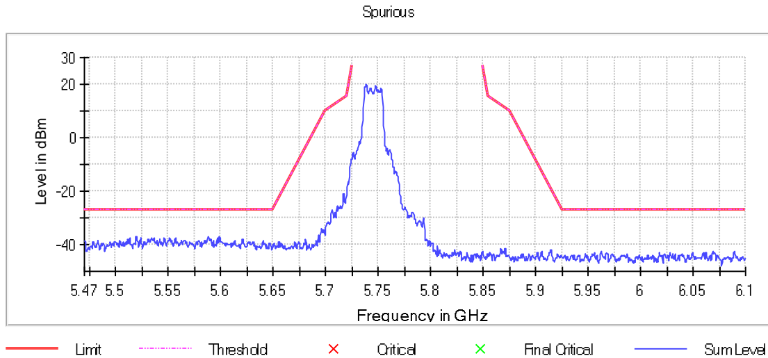
Graph 1: 20 MHz 5745 MHz
