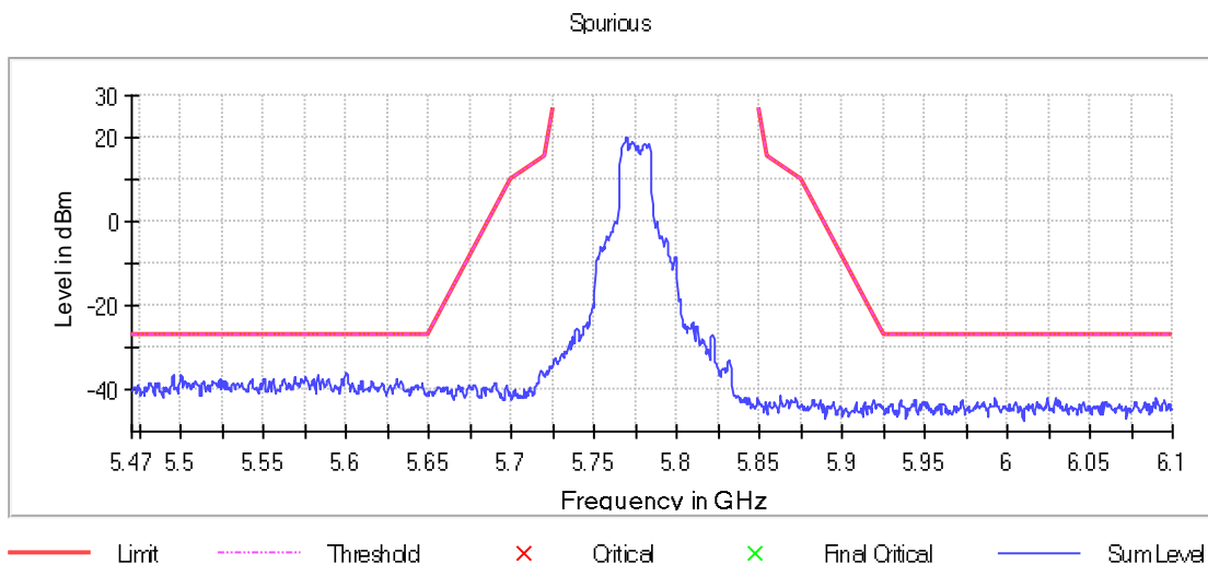
Graph 2: 20 MHz 5775 MHz
