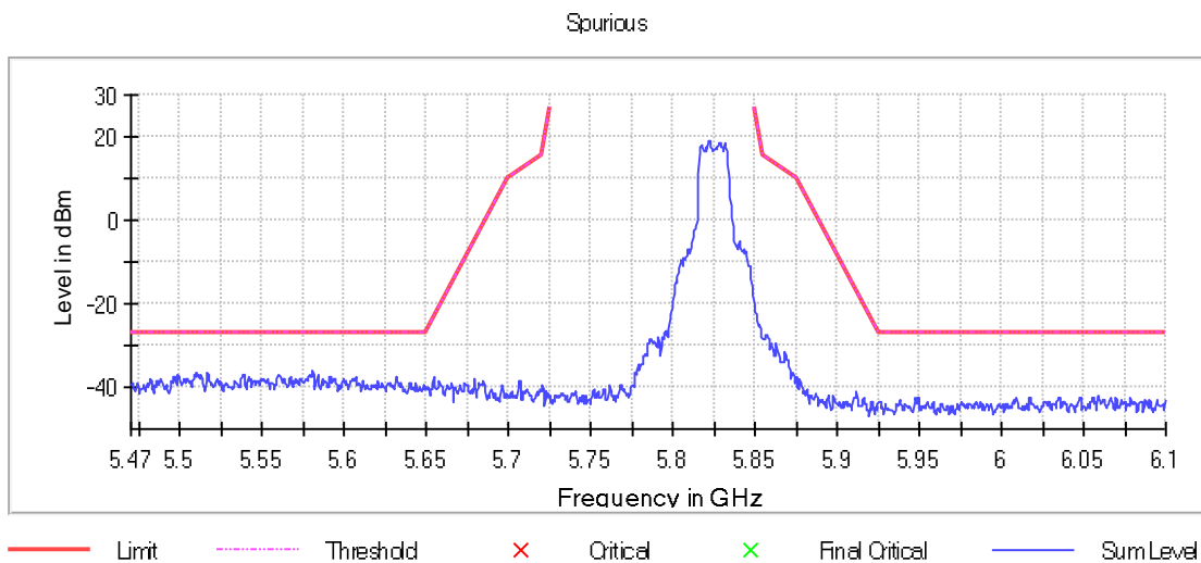
Graph 3: 20 MHz 5825 MHz
