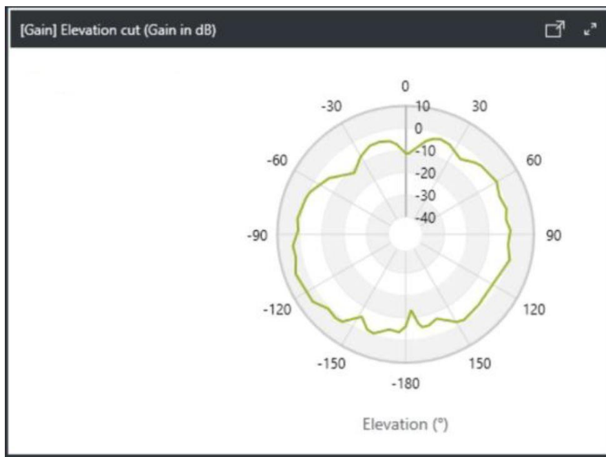
Figure 1: Internal Antenna Elevation Plot Greater Than 30-Degrees from Horizon
