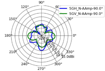
Azimuth
