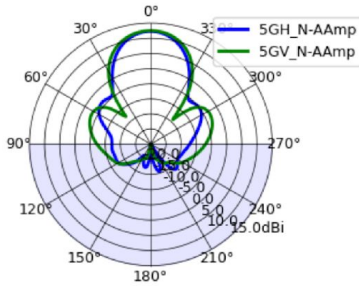
Elevation - 0.0°
