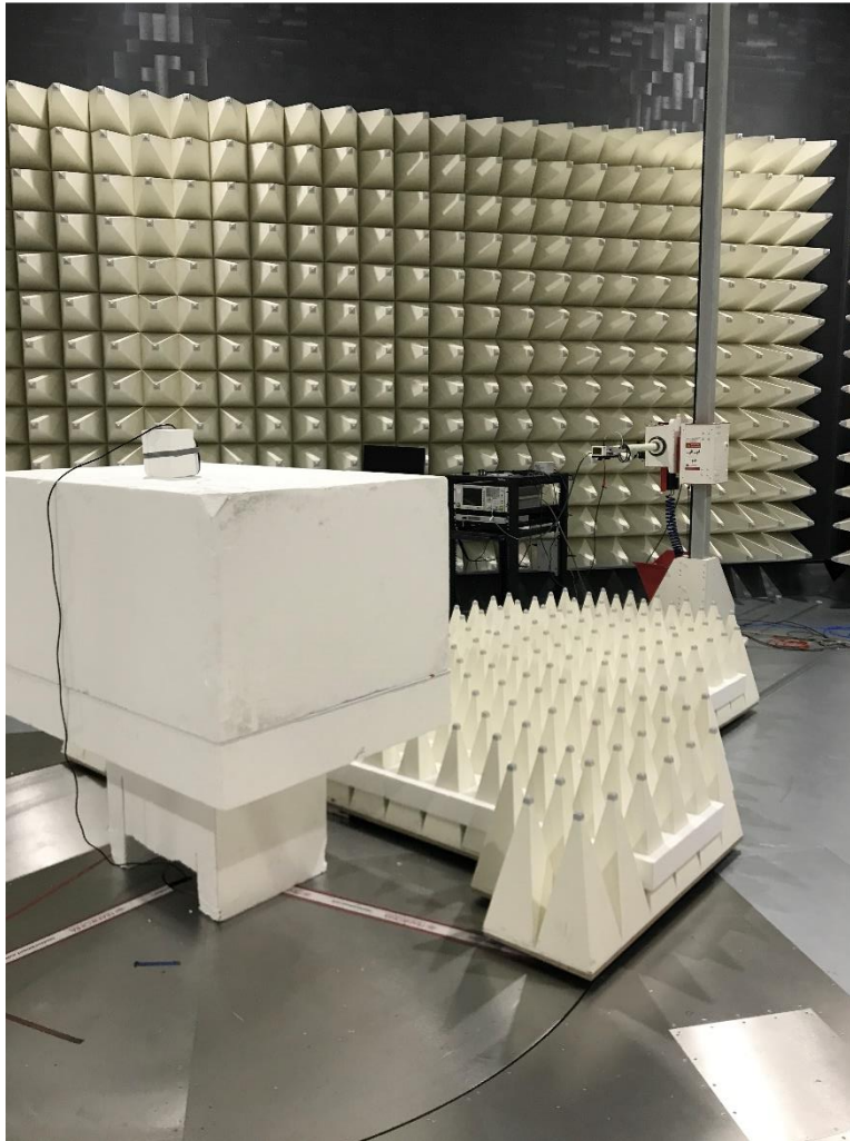
Photograph 3: Test Set Up Radiated Emissions 17 – 40 GHz
