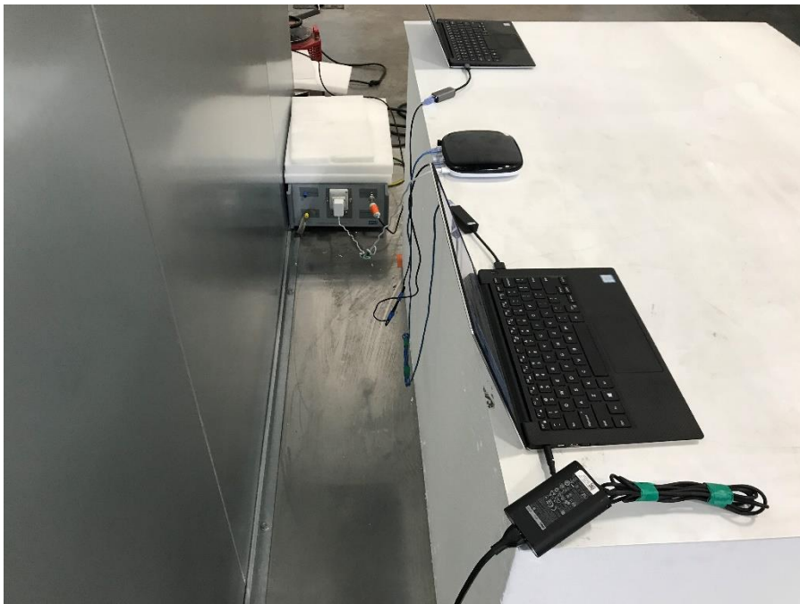
Photograph 5: Back Test Set Up AC Mains Conducted Emissions
