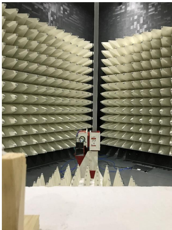
Photograph 2: Back View Test Set Up Radiated Emissions
