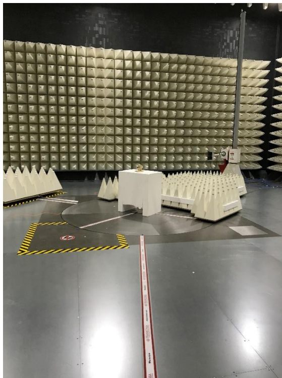
Photograph 1: Side View Test Set Up Radiated Emissions
