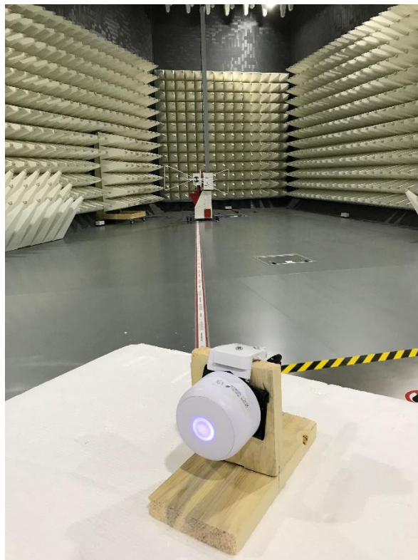
Photograph 3: Front View Test Set Up Radiated Emissions
