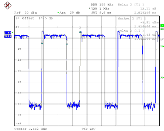
Modulation Type: \pi/4 -DQPSK-DH3 Channel: 00
