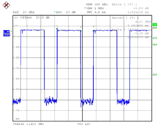
Modulation Type: GFSK-DH3 Channel: 00
