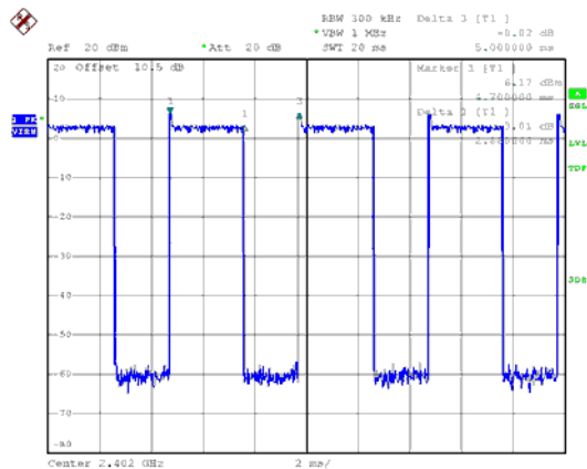
Modulation Type: 8DPSK-DH5 Channel: 00
