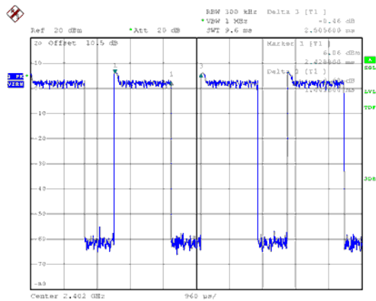
Modulation Type: 8DPSK-DH3 Channel: 00
