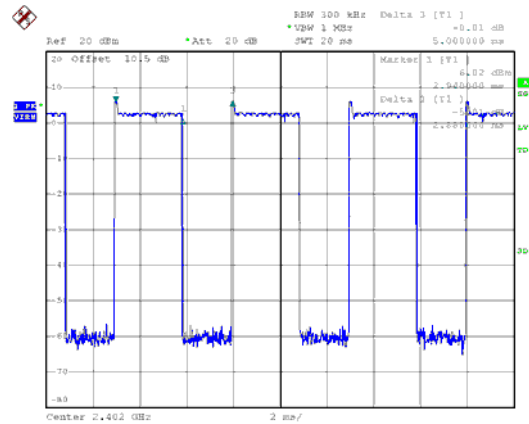
Modulation Type: \pi/4 -DQPSK-DH5 Channel: 00
