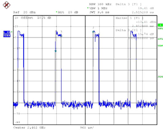
Modulation Type: 8DPSK-DH1 Channel: 00
