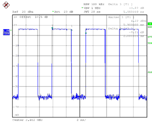
Modulation Type: GFSK-DH5 Channel: 00
