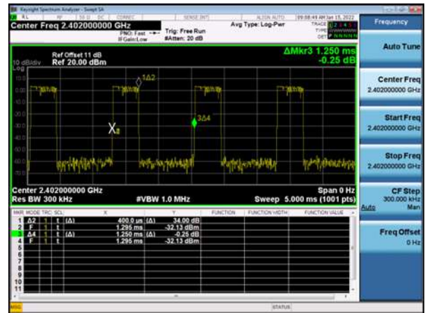
Modulation Type: π/4-DQPSK-DH3 Channel: 00
