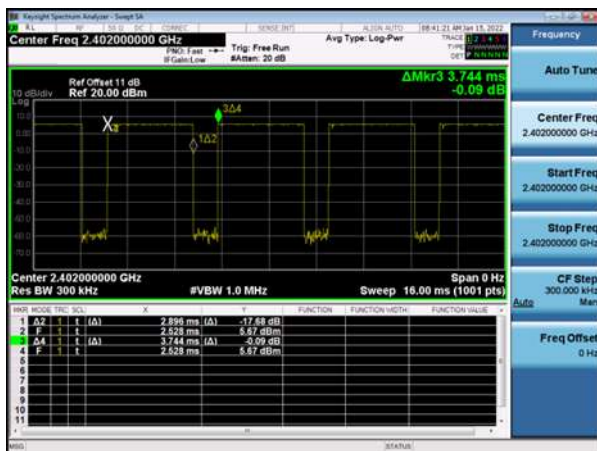
Modulation Type: GFSK-DH5 Channel: 00
