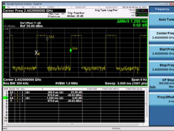
Modulation Type: GFSK-DH3 Channel: 00
