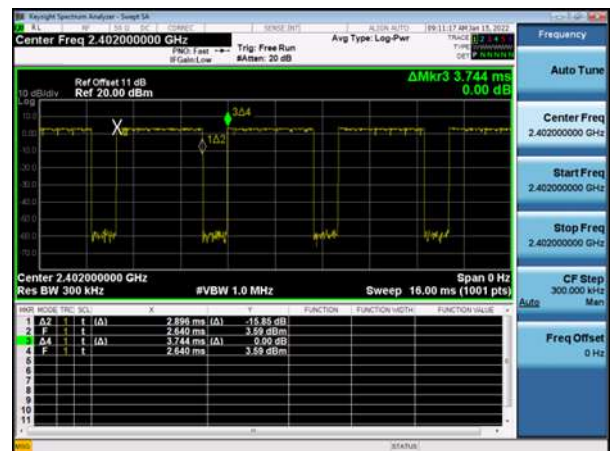
Modulation Type: π/4-DQPSK-DH5 Channel: 00
