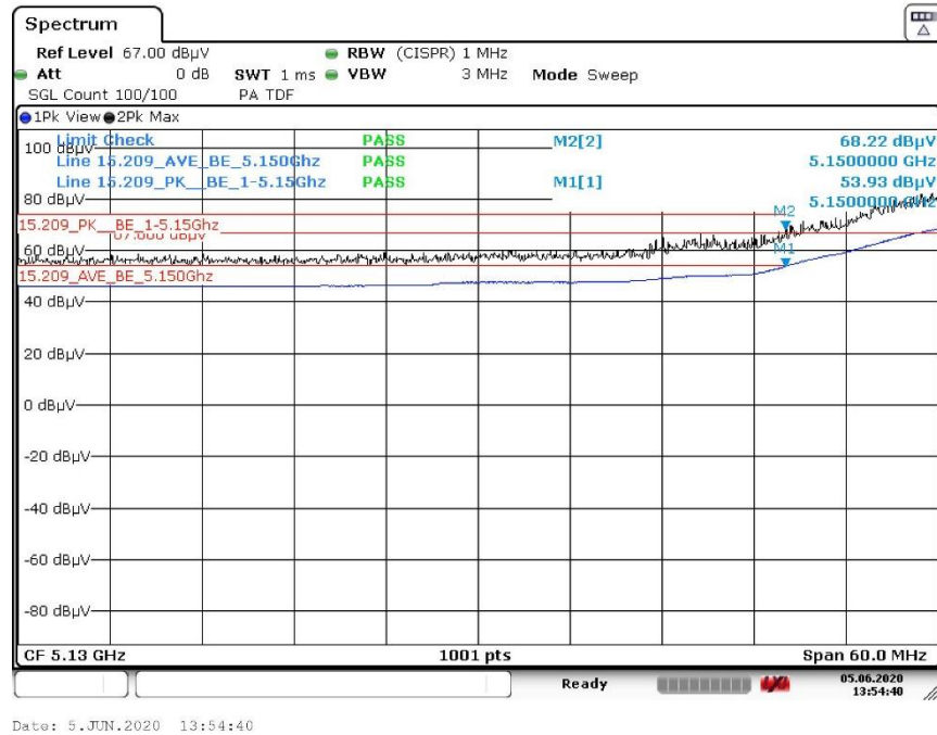
Plot 2: Transmitting on 5180 MHz n mode
