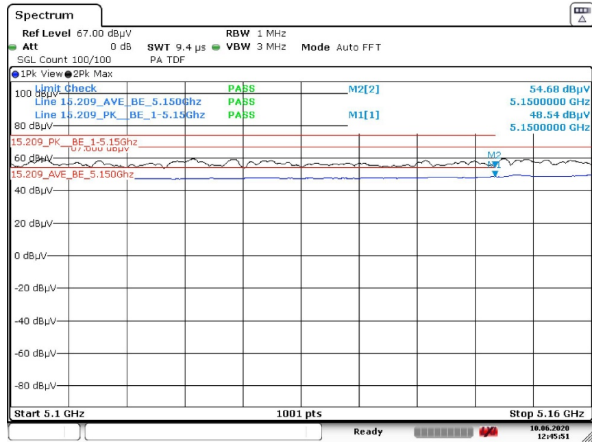
Plot 2: Transmitting on 5200 MHz a mode 20 MHz ch
