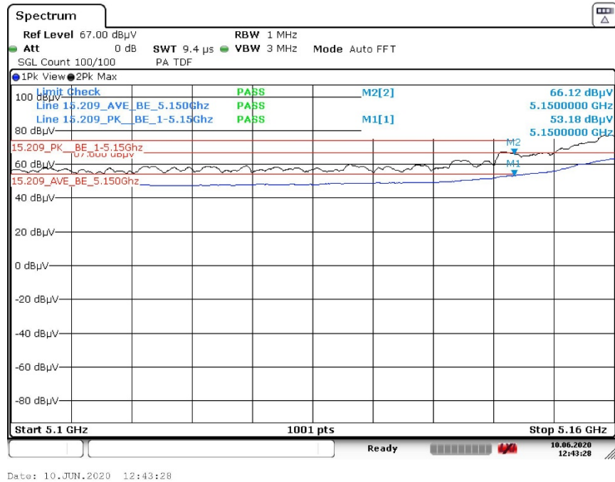
Plot 3 Transmitting on 5180 MHz ac mode 20 MHz ch
