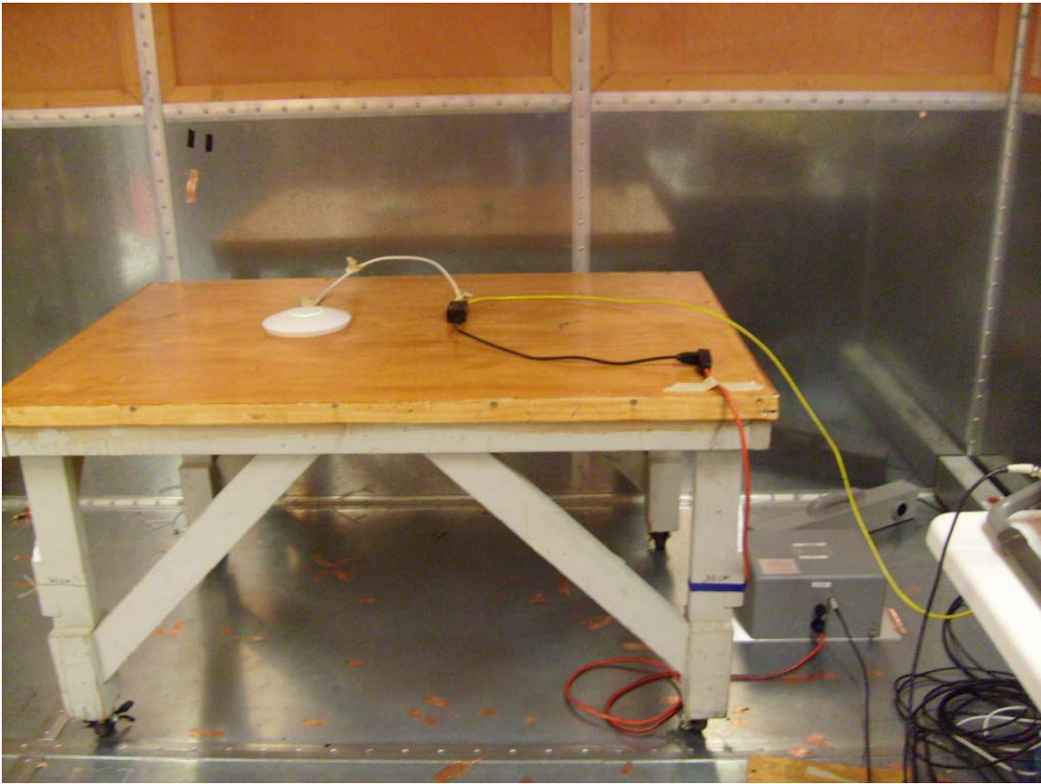
Photograph 3. Conducted Emissions
