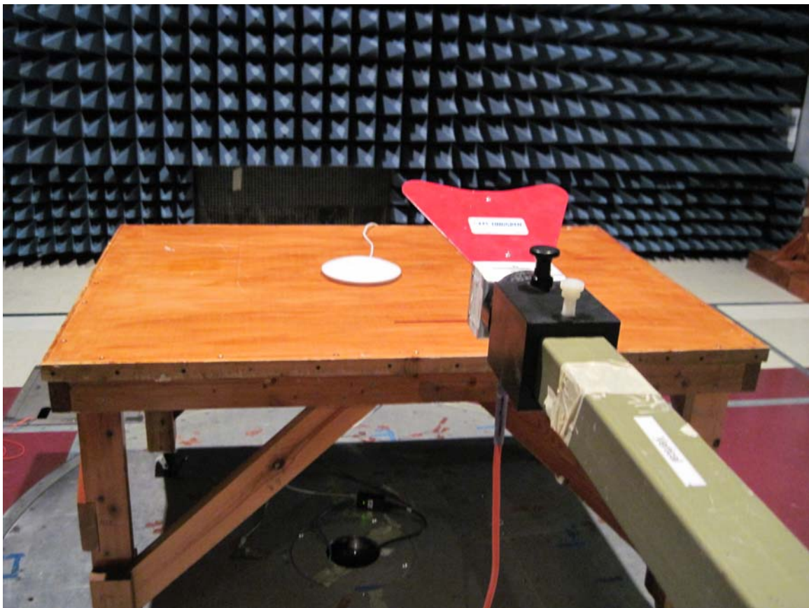
Photograph 2. Radiated Spurious Emissions @ 1 m
