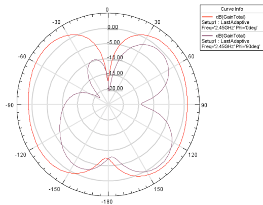
Elevation Cuts
