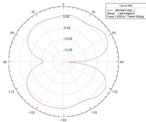
Azimuth Cut
