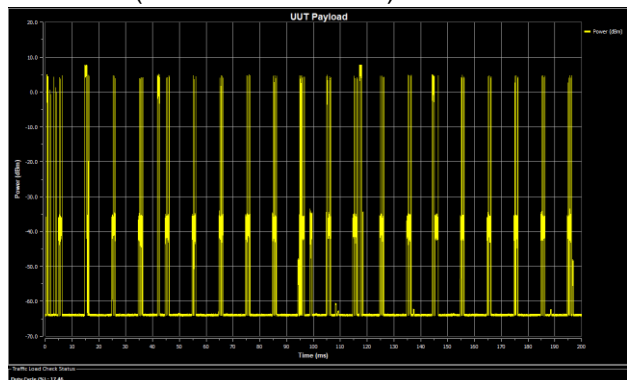
Modulation Type:802.11ac VHT80 Time On/ (Time On + Off Time) =17.46%
