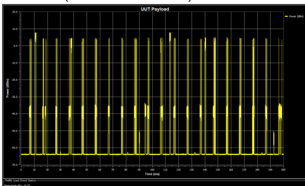
Modulation Type:802.11ac VHT80 Time On/ (Time On + Off Time) =17.27%
