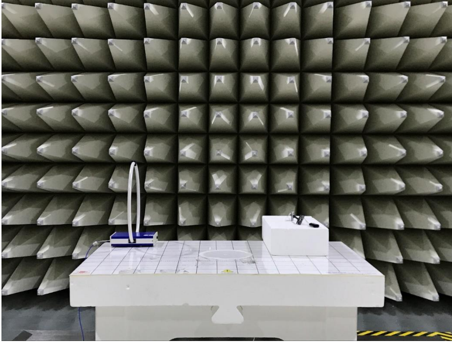
Photograph 3: Test Setup NFC Configuration
