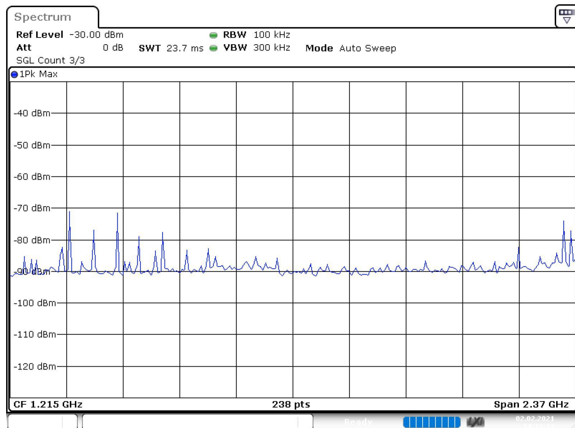
Spurious Connector 1_0
