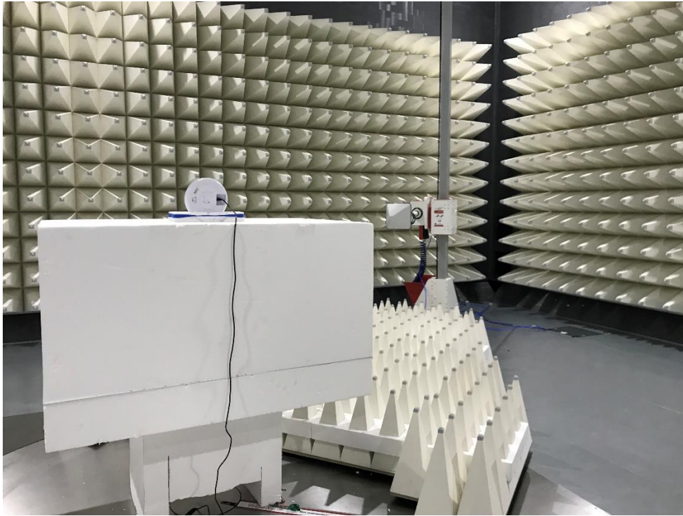
Photograph 3: Back View Test Set Up Radiated Emissions 1 – 16 GHz
