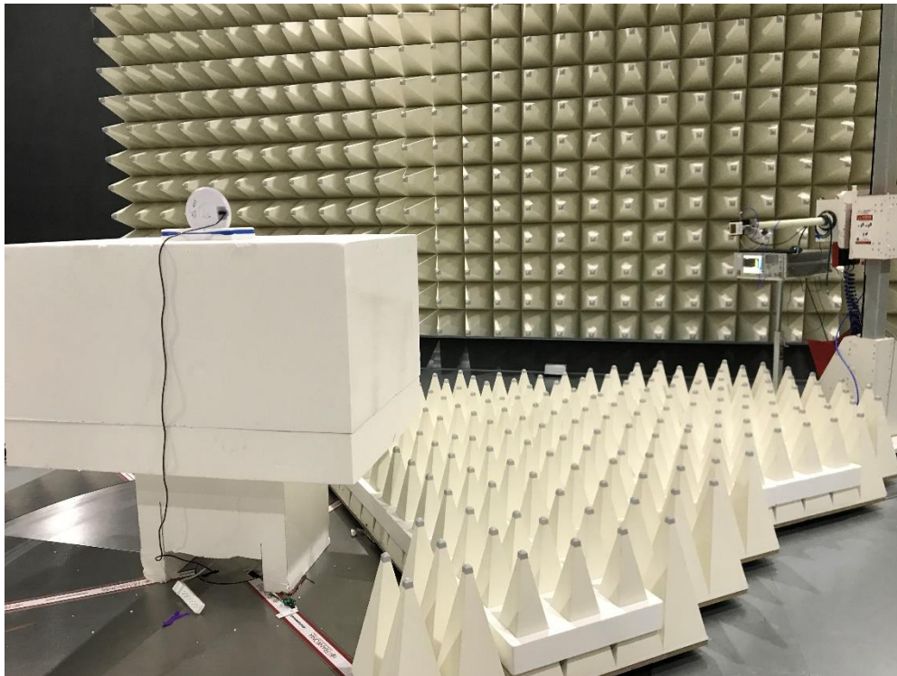
Photograph 4: Side View Test Set Up Radiated Emissions 16 – 40 GHz
