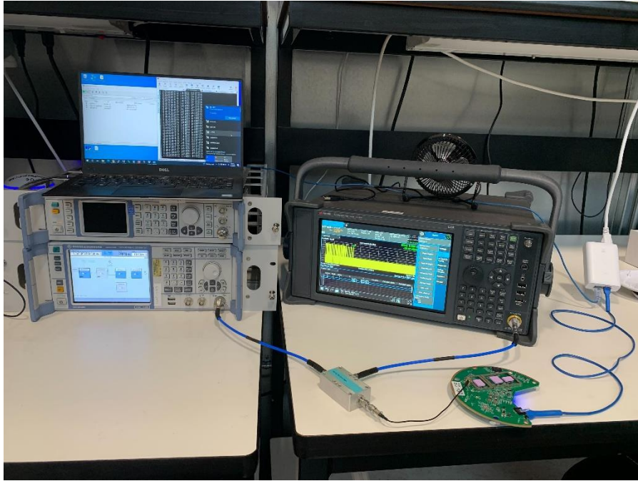
Photograph 5: View Test Set DFS
