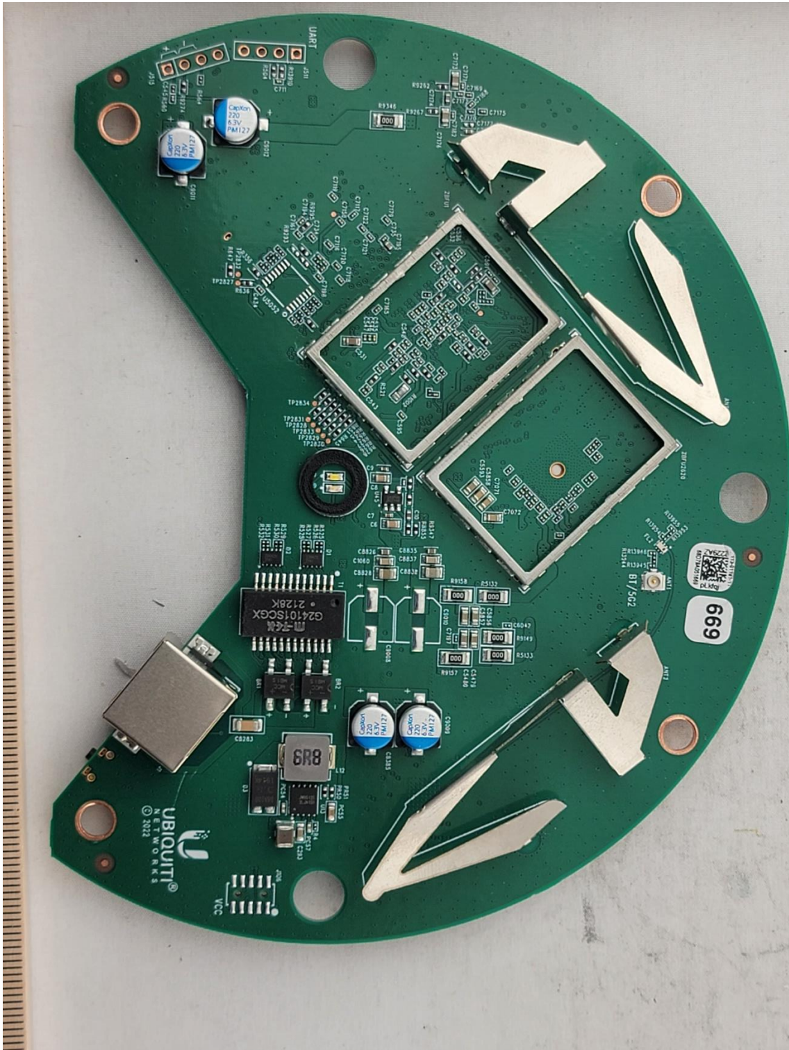
Photograph 2: Front View of DUT Shields removed
