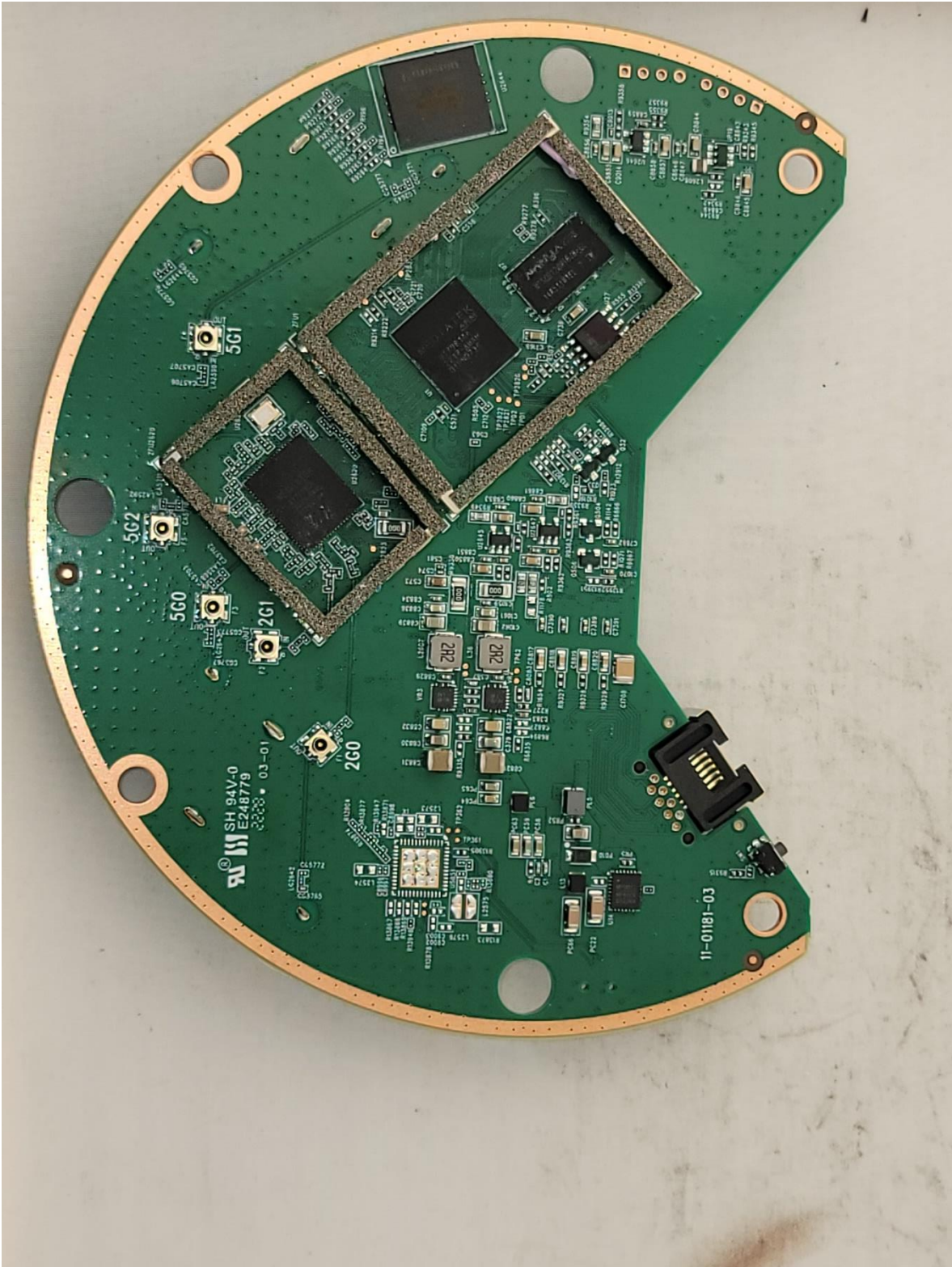
Photograph 3: Rear View of DUT
