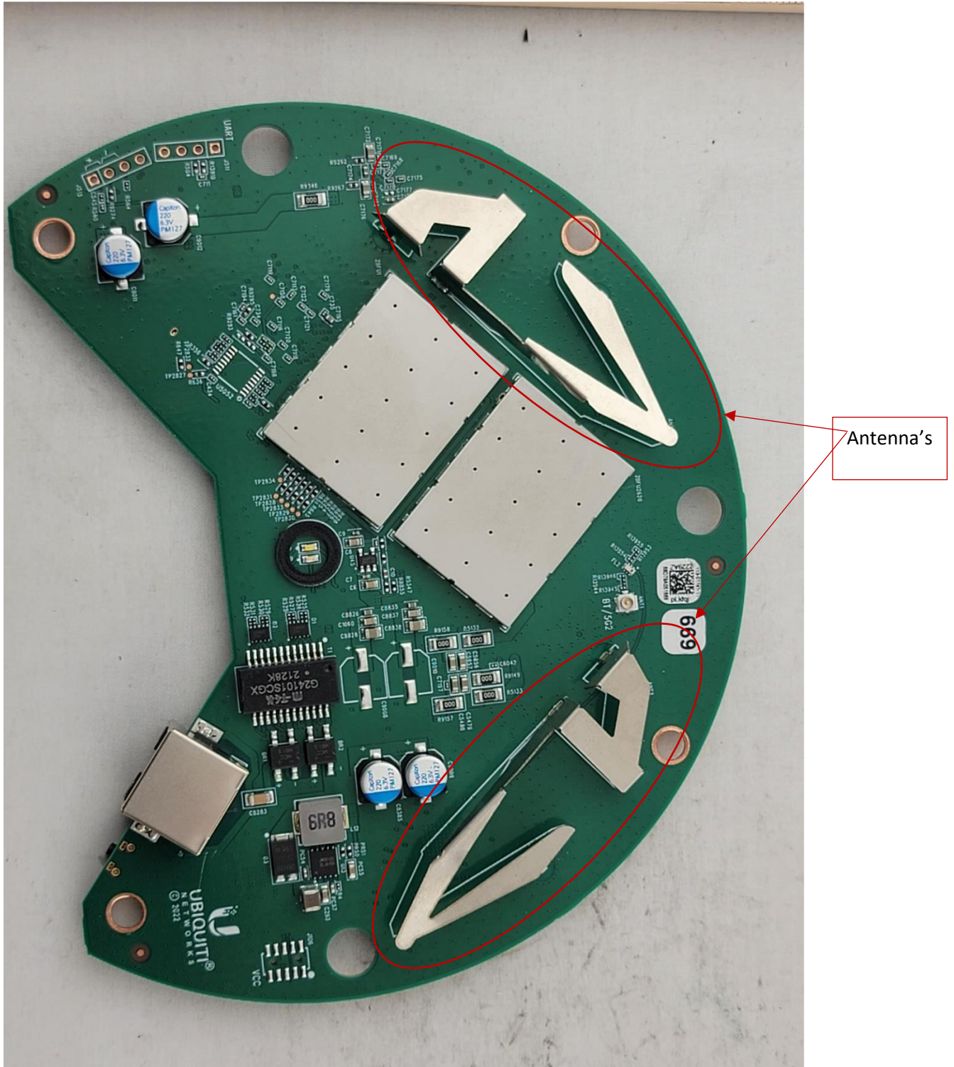
Photograph 1: Front View of DUT Shields in place
