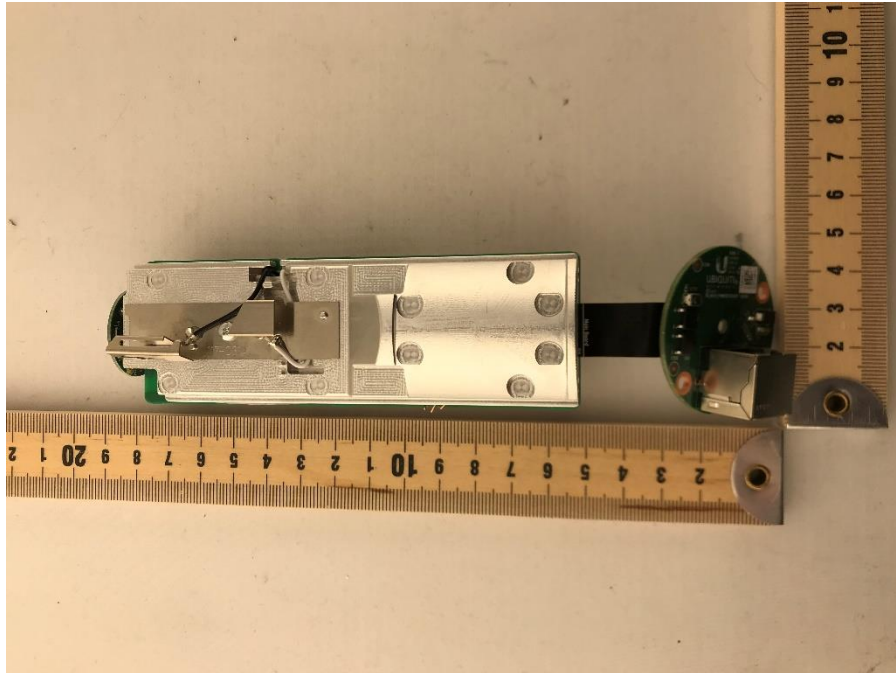
Photograph 1: Front View of DUT with Heat Sink
