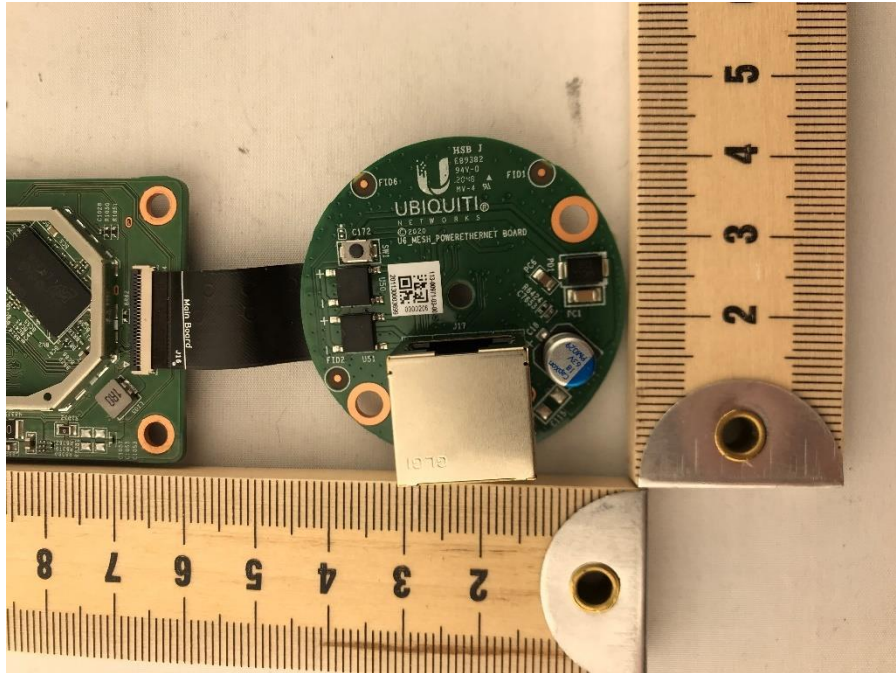
Photograph 9: Front View of DUT Ethernet Circuit Board
