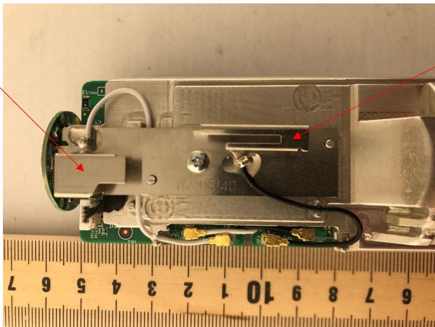
Photograph 6: Close-Up of Antennas – Back View
