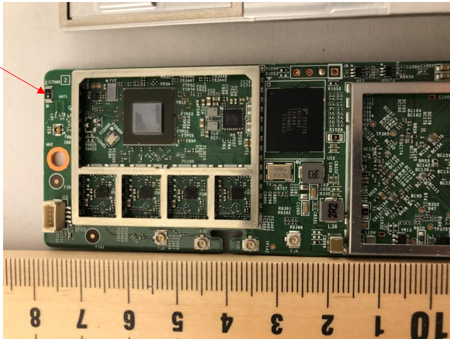
Photograph 11: Close-Up View of RF Circuitry
