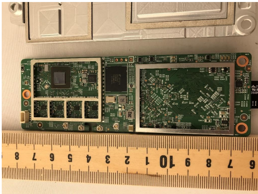
Photograph 8: Back View of Main DUT Circuit Board
