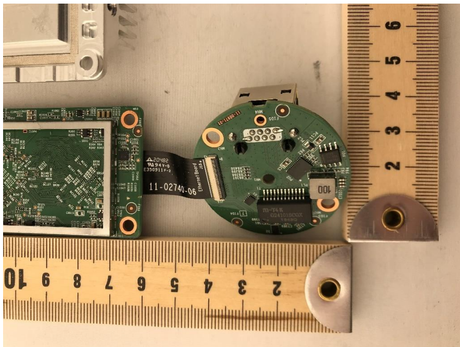
Photograph 10: Back View of DUT Ethernet Circuit Board
