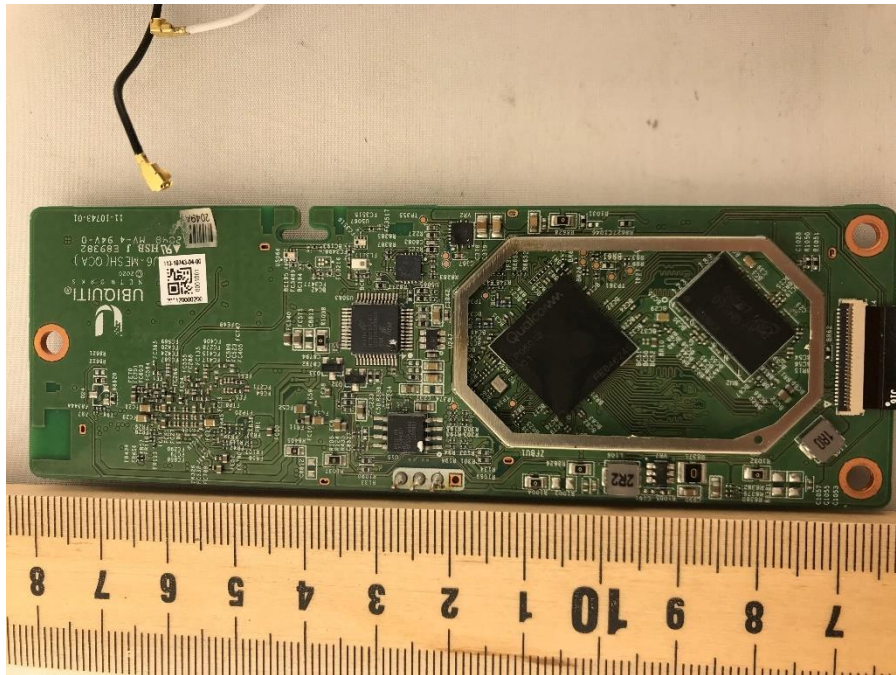
Photograph 7: Front View of Main DUT Circuit Board
