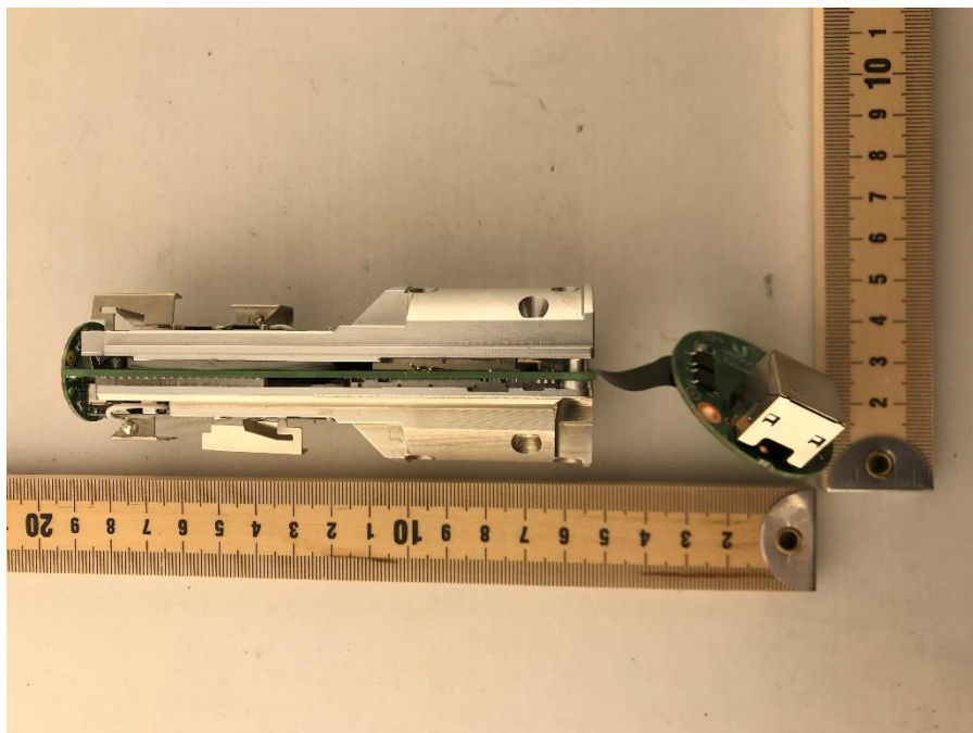
Photograph 2: Side View of DUT with Heat Sink
