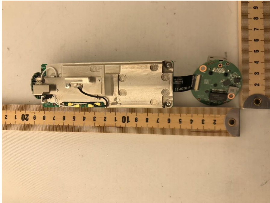
Photograph 3: Back View of DUT with Heat Sink
