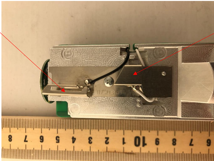
Photograph 5: Close-Up of Antennas – Front View
