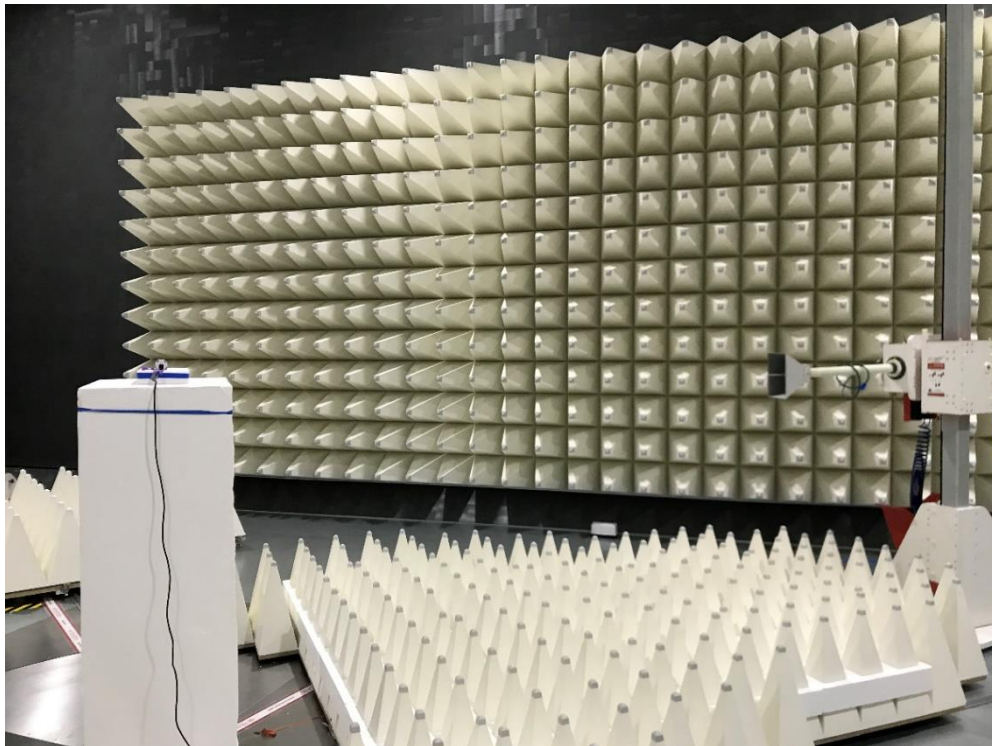
Photograph 2: Side View Test Set Up Radiated Emissions
