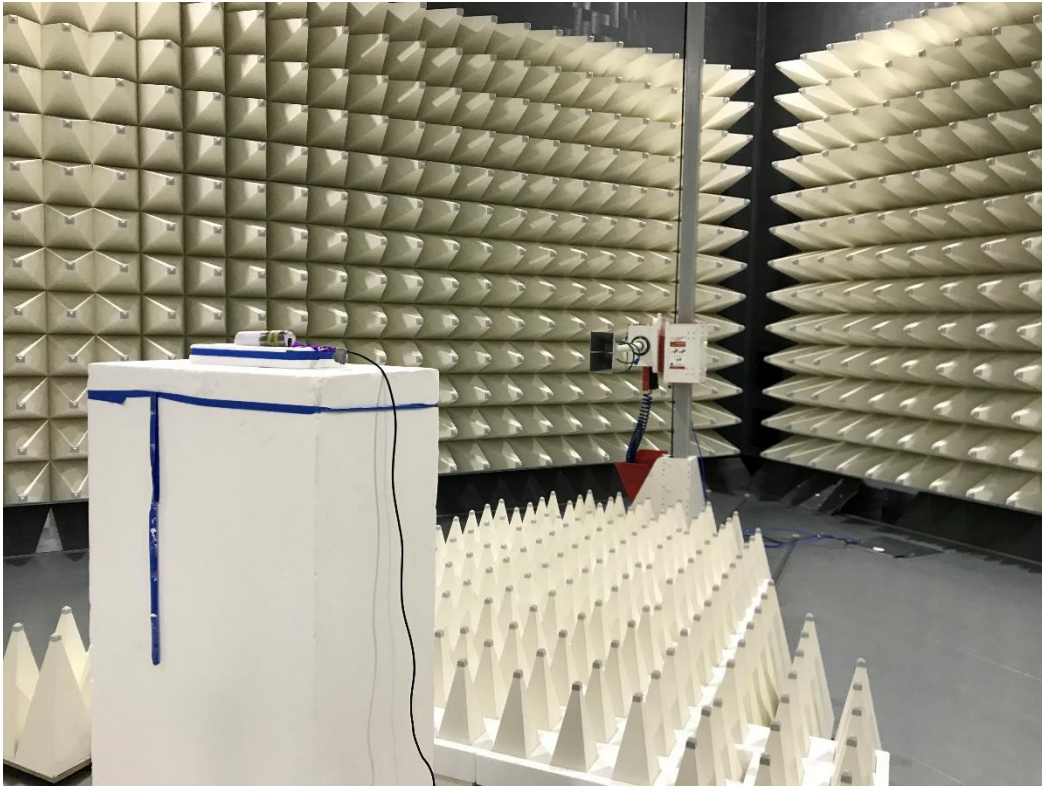
Photograph 3: Front View Test Set Up Radiated Emissions
