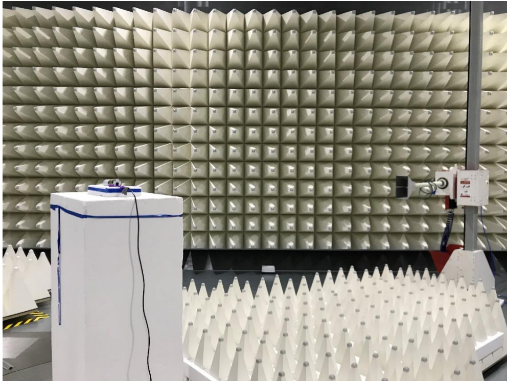
Photograph 1: Side View Test Set Up Radiated Emissions
