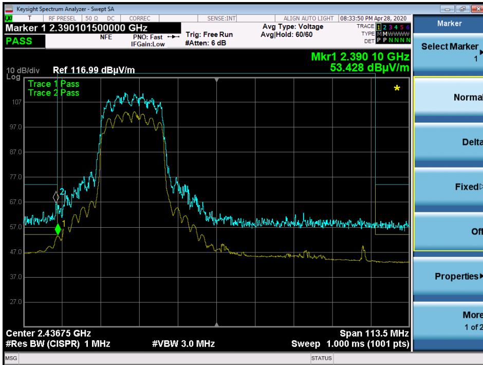
Graph 9: Lower Band Edge Plot N mode 20 MHz
