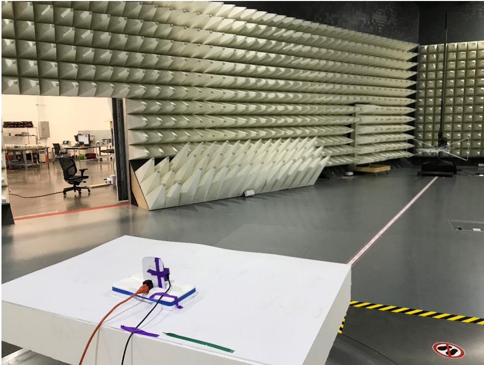
Photograph 1: Back View Test Set Up Radiated Emissions 30 – 1000 MHz
