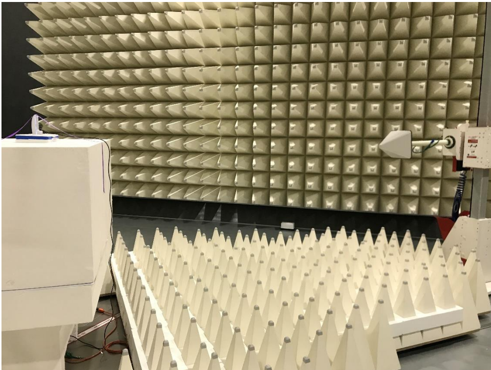
Photograph 2: Side View Test Set Up Radiated Emissions 1 – 16 GHz
