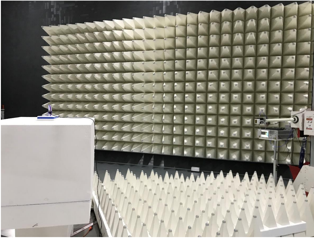
Photograph 3: Side View Test Set Up Radiated Emissions 16 – 40 GHz
