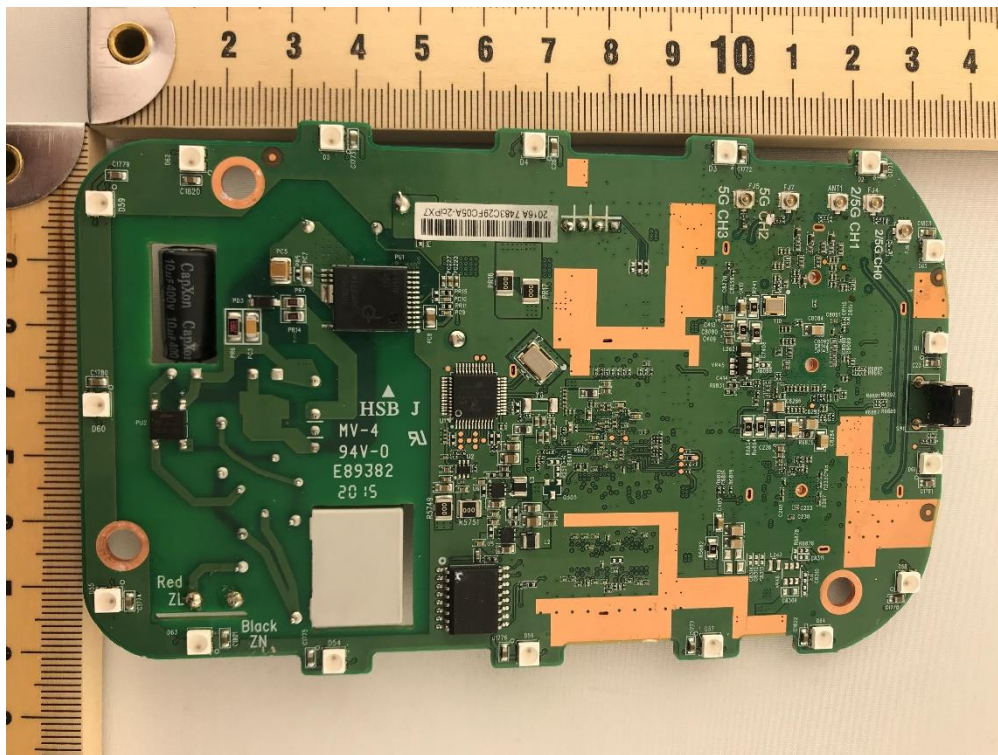
Photograph 1: Top View of Circuit Board
