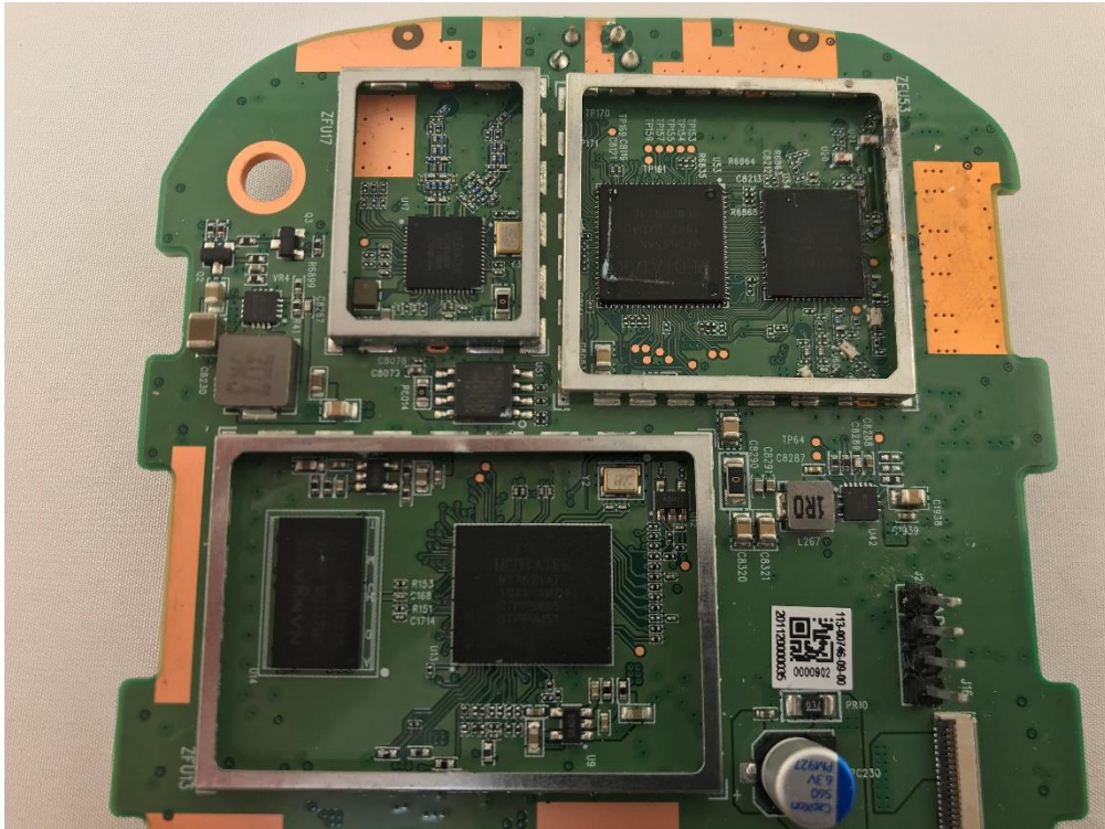
Photograph 3: Close up View of Circuit Board Showing RF Chips
