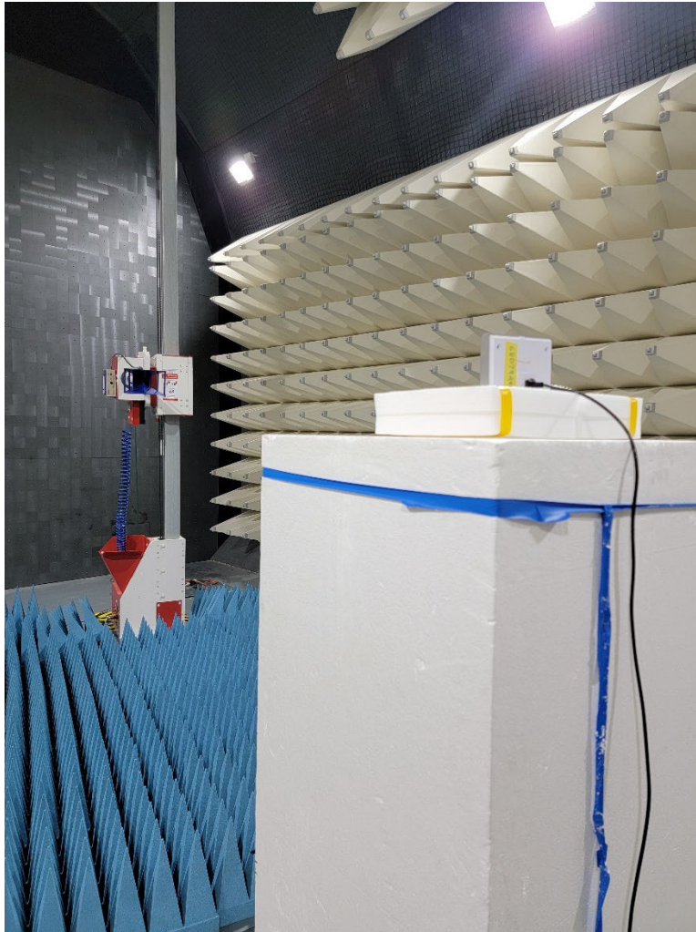
Radiated Emissions 1-17GHz
