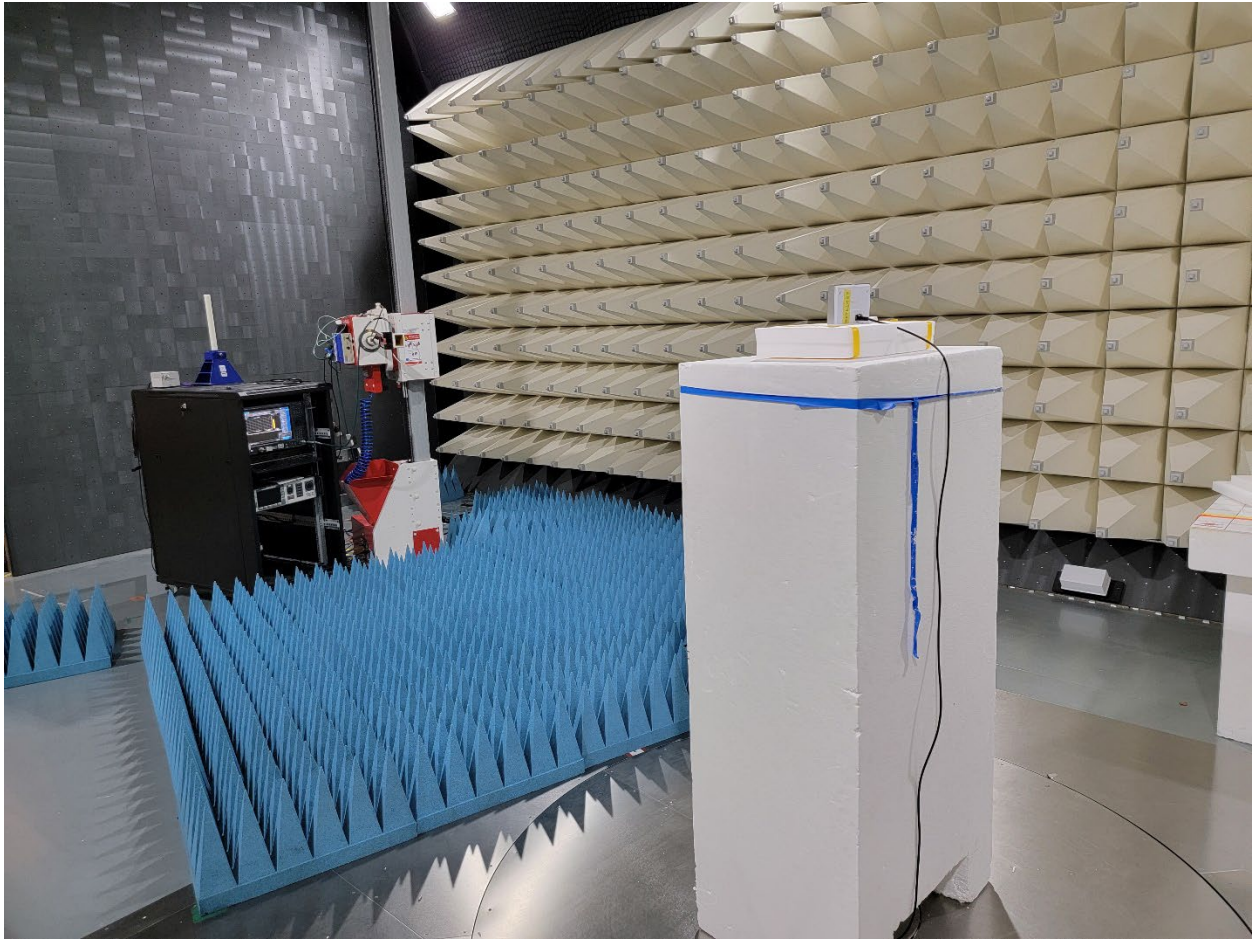
Radiated Emissions 17-40GHz
