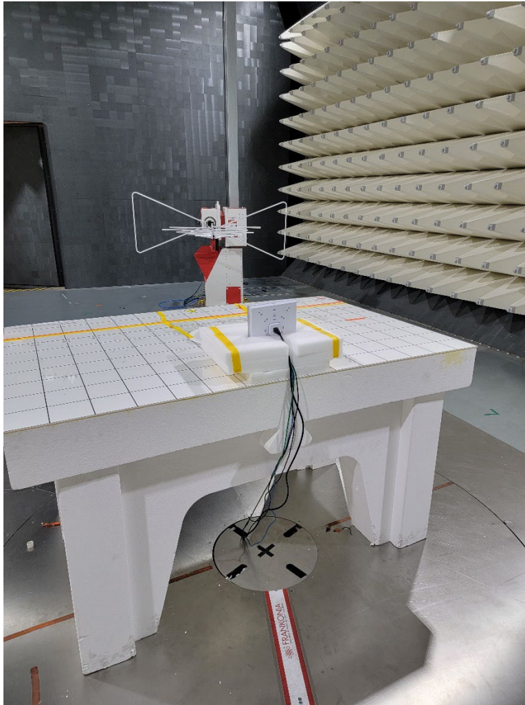
Radiated Emissions 30-1000MHz
