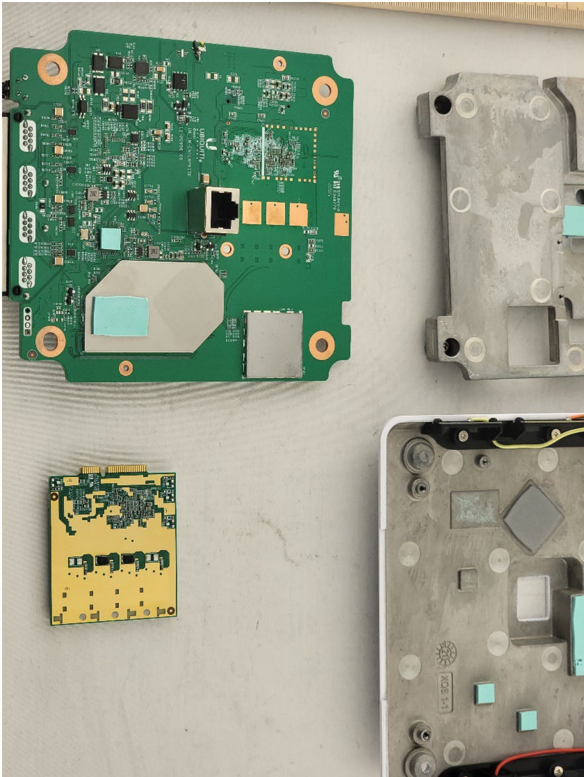
DUT Disassembled
