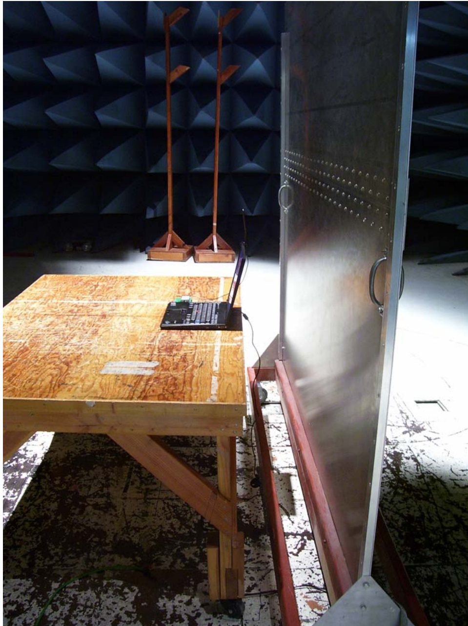
Photograph 3. Conducted Emissions Test Setup
