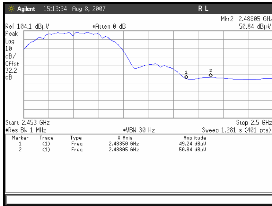
Plot 15. 802.11/b radiated restricted band 2483.5 – 2500MHz Avg
