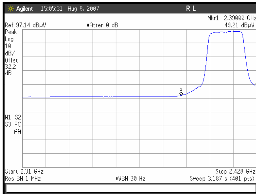
Plot 17. 802.11/g radiated restricted band 2310- 2390 MHz Avg
