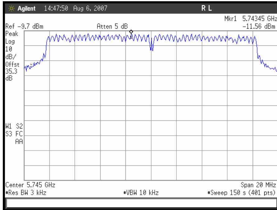
Plot 53. 802.11/a – Low Ch Peak Power Spectral Density
