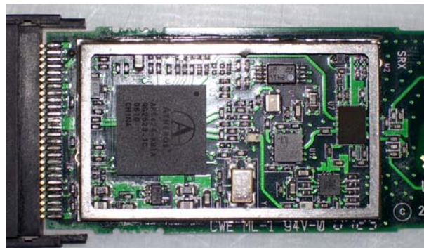
Photograph 1. Ubiquiti Networks SRX
