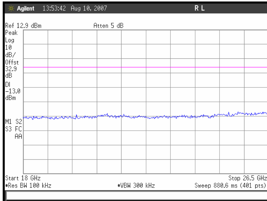
Plot 23. 802.11/b – Mid Channel Conducted Emissions 18 – 26.5GHz
