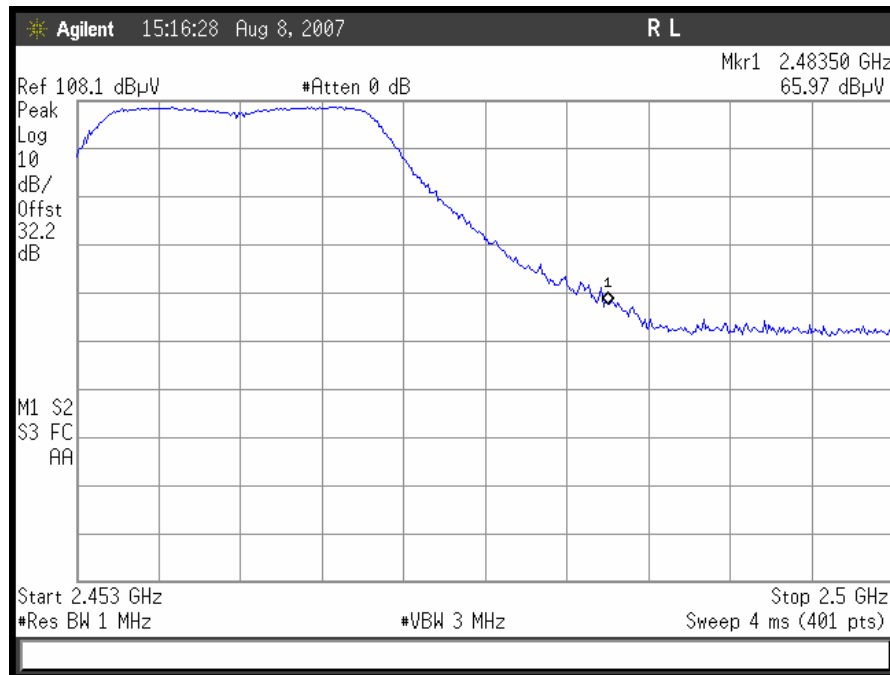
Plot 18. 802.11/g radiated restricted band 2483.5 – 2500MHz Peak
