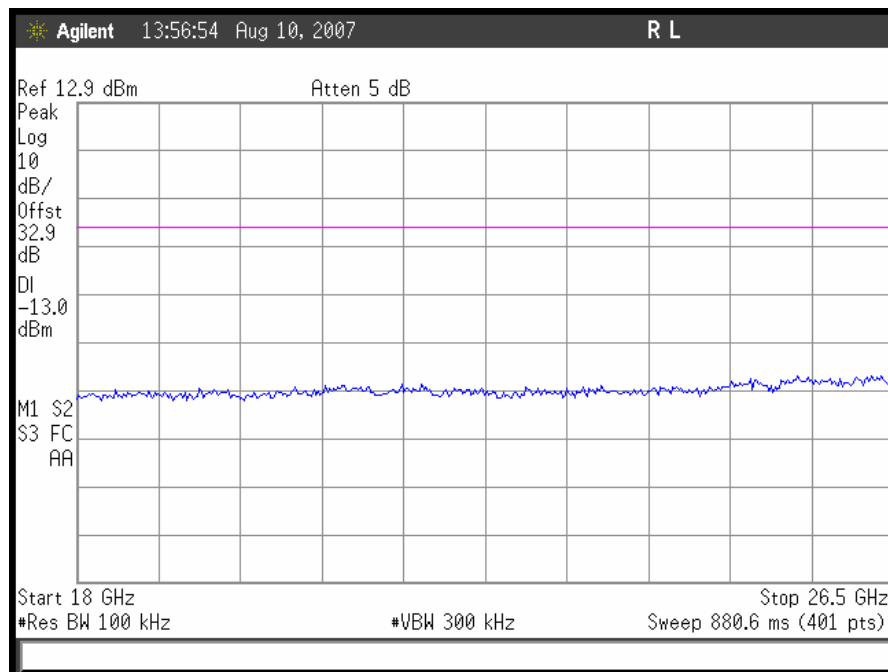
Plot 29. 802.11/g – Mid Channel Conducted Emissions 18 – 26.5GHz
