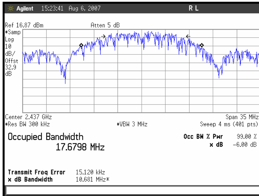
Plot 4. 802.11/b Mid Ch Occupied Band Width
