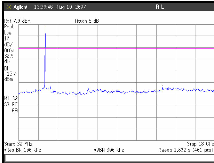
Plot 30. 802.11/g – High Channel Conducted Emissions 30MHz- 18GHz
