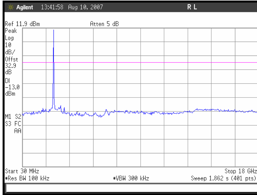
Plot 20. 802.11/b – Low Channel Conducted Emissions 30MHz - 18GHz
