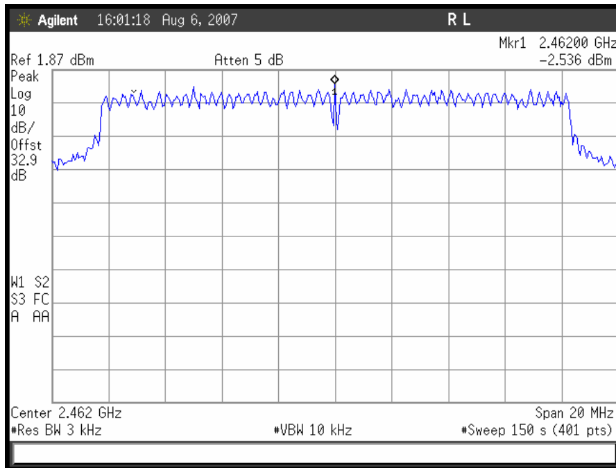
Plot 52. 802.11/g – High Ch Peak Power Spectral Density
