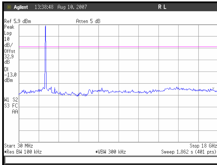
Plot 28. 802.11/g – Mid Channel Conducted Emissions 30MHz – 18GHz
