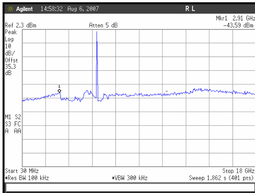
Plot 35. 802.11/a – Mid Channel Conducted Emissions 30MHz – 18GHz
