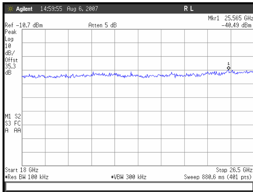
Plot 39. 802.11/a – High Channel Conducted Emissions 18-26.5GHz
