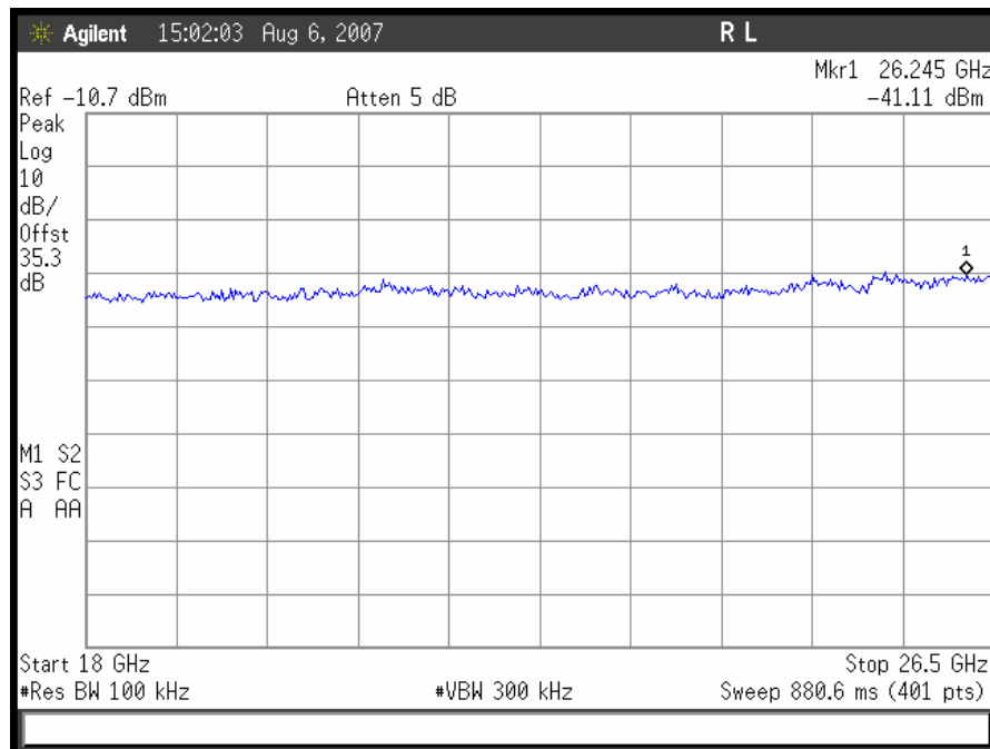
Plot 33. 802.11/a – Low Channel Conducted Emissions 18 -26.5GHz
