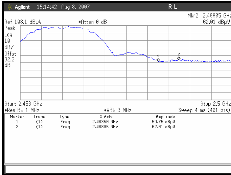
Plot 14. 802.11/b radiated restricted band 2483.5 – 2500MHz Peak
