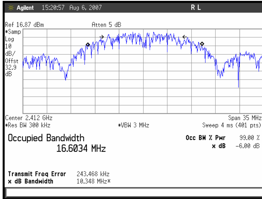
Plot 3. 802.11/b Low Ch Occupied Band Width.
