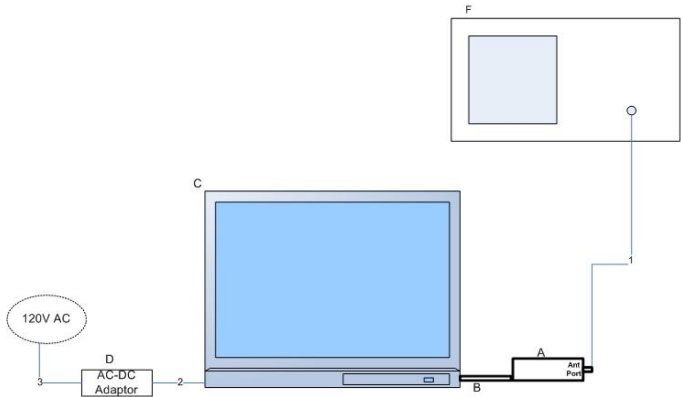
Figure 2. Block Diagram of Test Configuration (Conducted Emissions)
