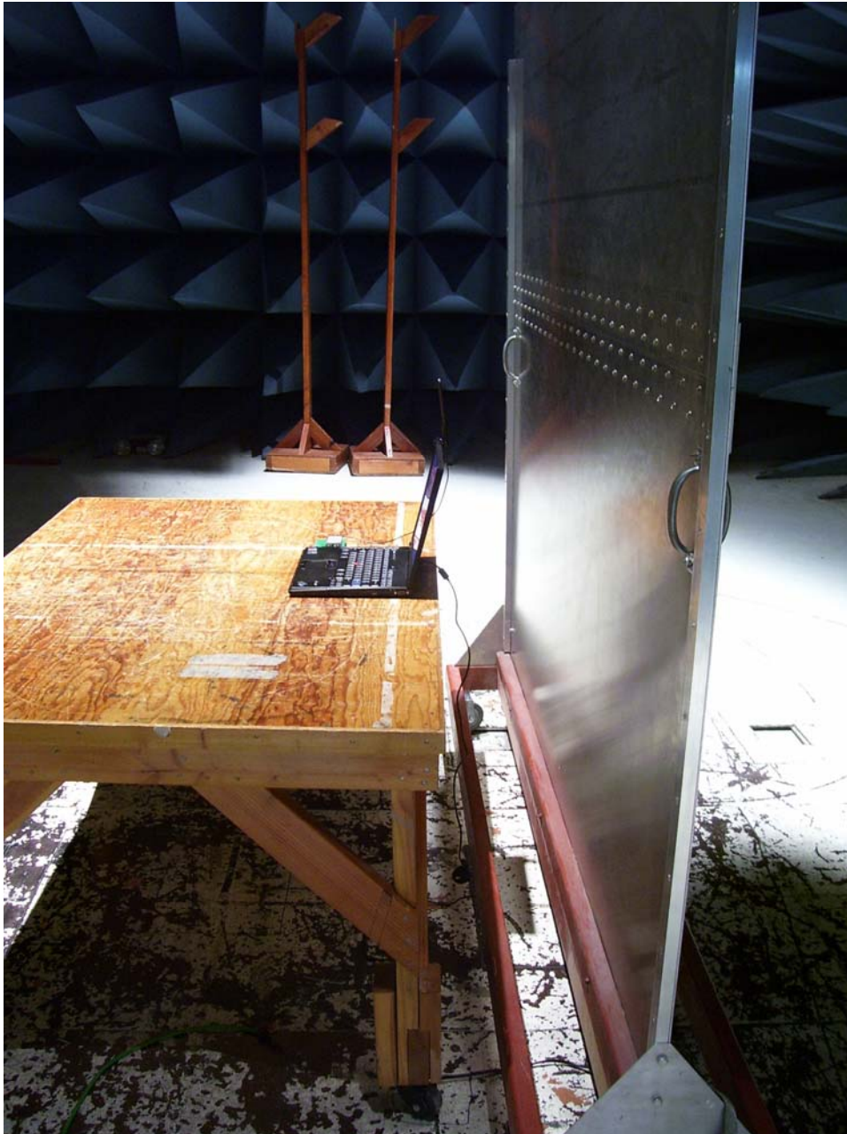
Photograph 4. Conducted Emissions Test Setup
