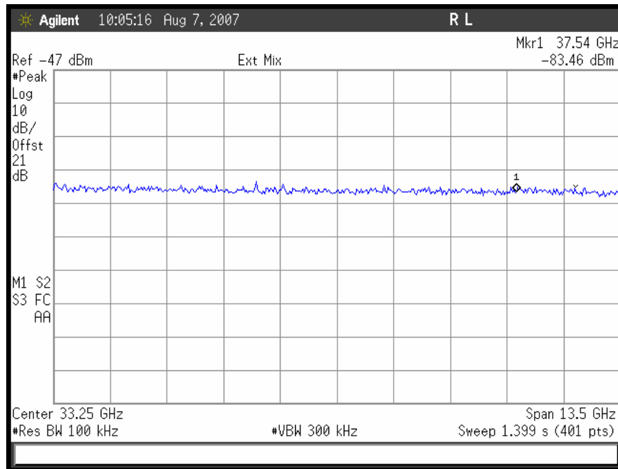
Plot 37. 802.11/a – Mid Channel Conducted Emissions 26.5 – 40GHz
