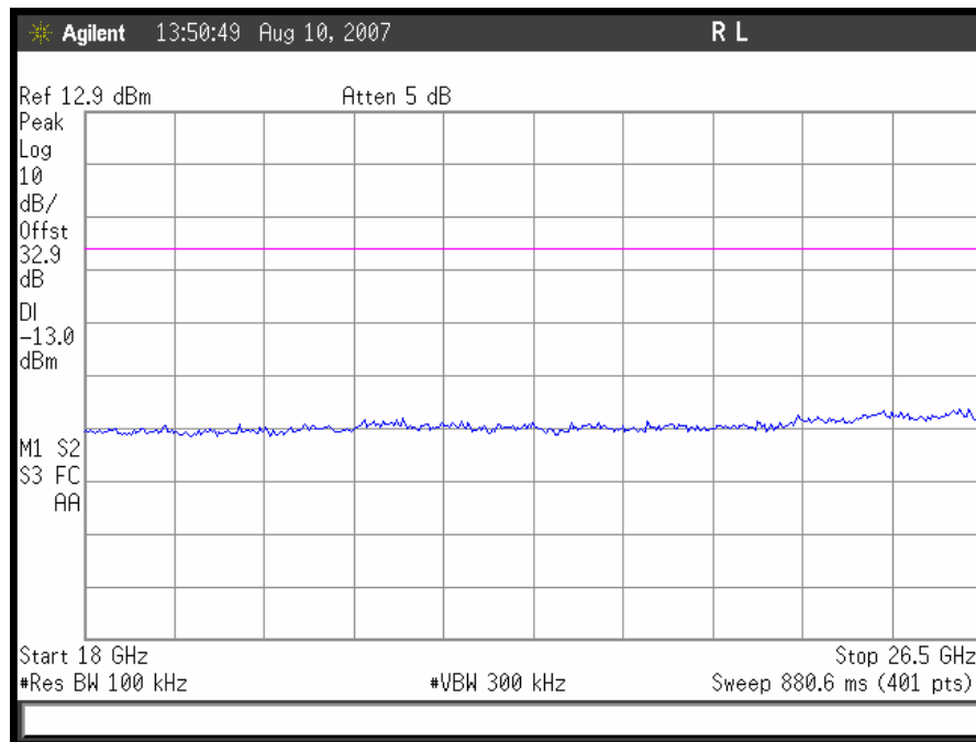
Plot 21. 802.11/b – Low Channel Conducted Emissions 18 – 26.5GHz
