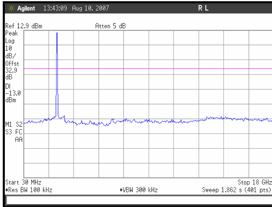
Plot 22. 802.11/b – Mid Channel Conducted Emissions 30MHz – 18GHz
