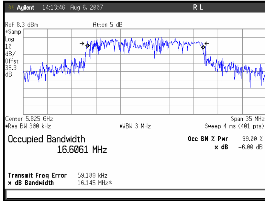
Plot 11. 802.11/a High Ch Occupied Band Width
