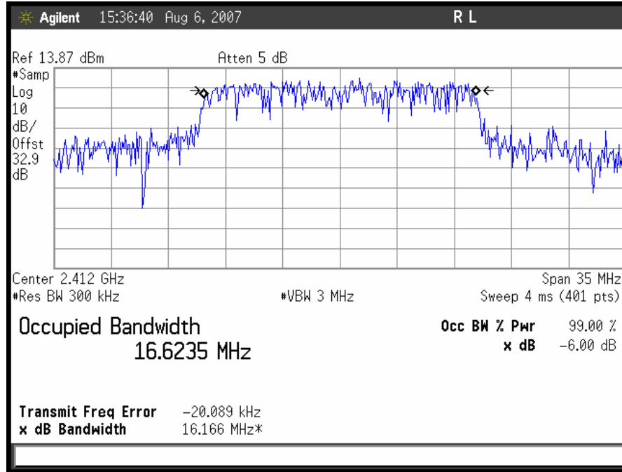
Plot 6. 802.11/g Low Ch Occupied Band Width
