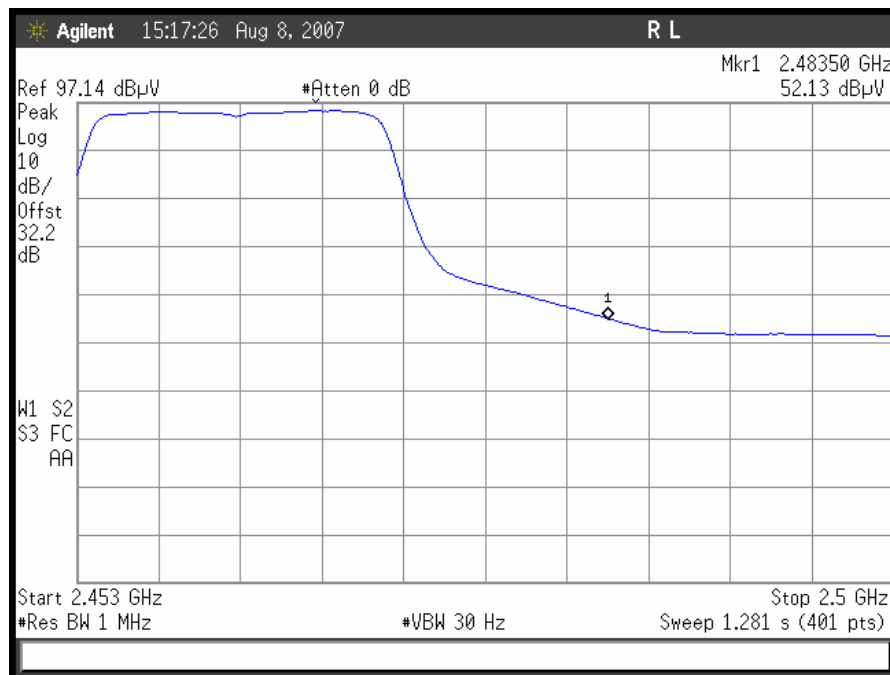
Plot 19. 802.11/g radiated restricted band 2483.5 – 2500MHz Avg
