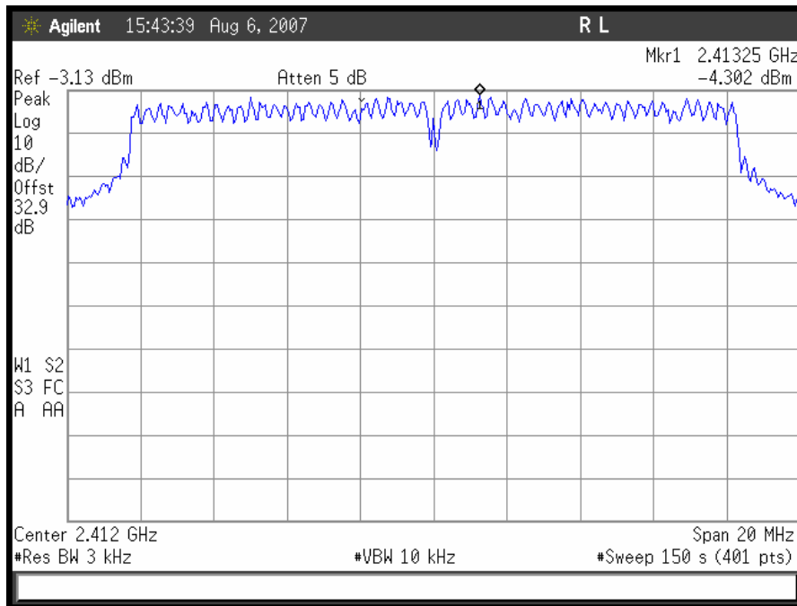
Plot 50. 802.11/g – Low Ch Peak Power Spectral Density
