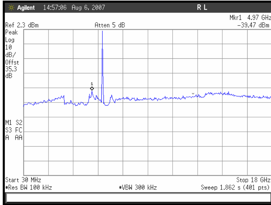
Plot 32. 802.11/a – Low Channel Conducted Emissions 30MHz- 18GHz
