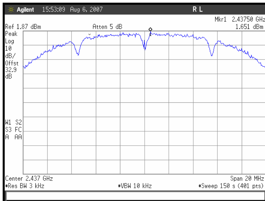
Plot 48. 802.11/b – Mid Ch Peak Power Spectral Density
