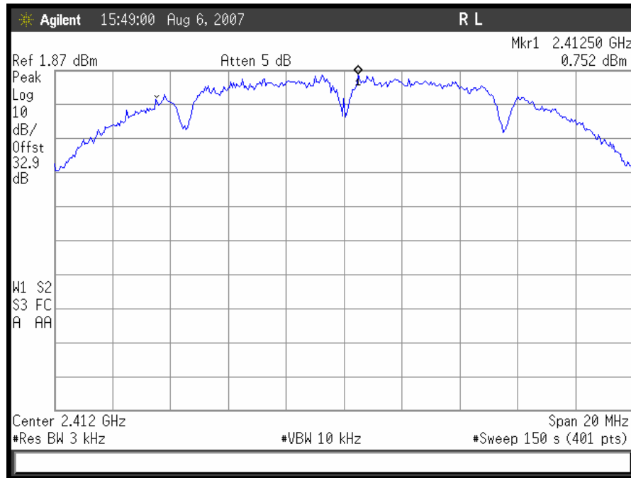
Plot 47. 802.11/b – Low Ch Peak Power Spectral Density
