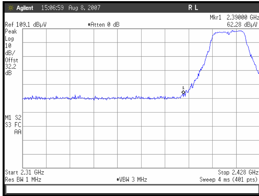
Plot 16. 802.11/g radiated restricted band 2310- 2390 MHz Peak
