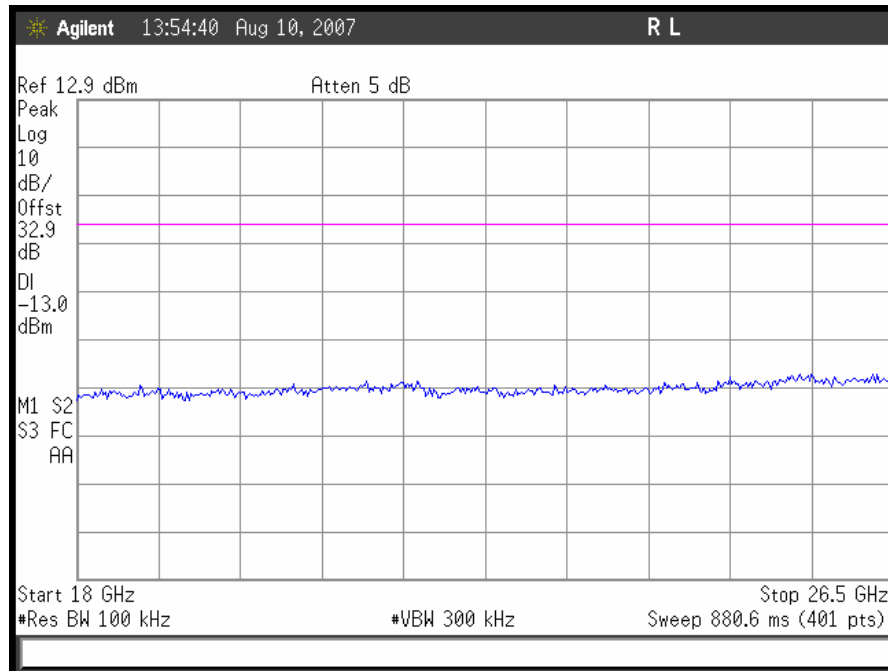
Plot 25. 802.11/b – High Channel Conducted Emissions 18 – 26.5GHz
