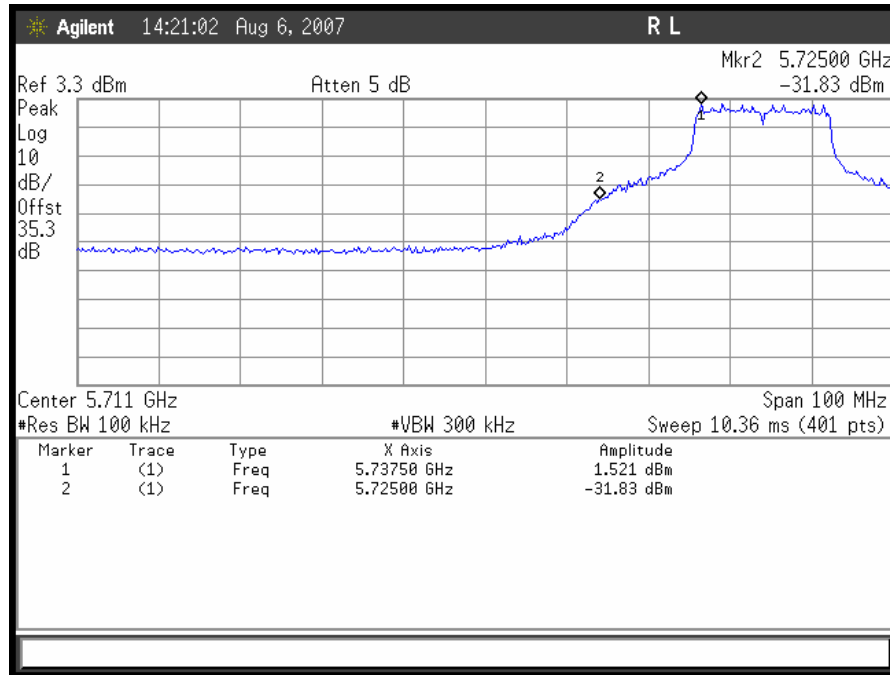
Plot 45. 802.11/a – Lower Band Edge
