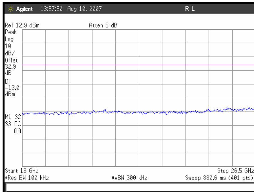
Plot 31. 802.11/g – High Channel Conducted Emissions 18 – 26.5GHz
