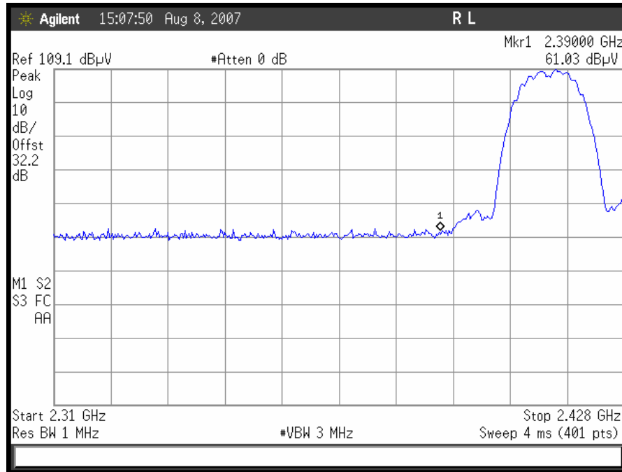
Plot 12. 802.11/b radiated restricted band 2310- 2390 MHz Peak
