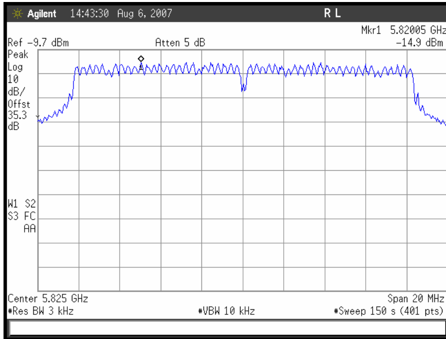
Plot 55. 802.11/a – High Ch Peak Power Spectral Density
