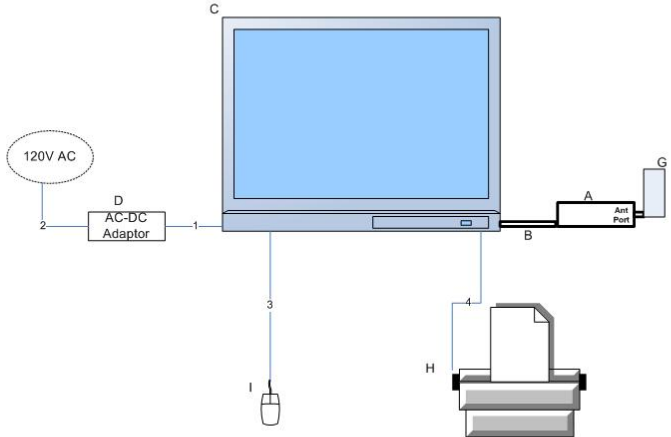
Figure 1. Block Diagram of Test Configuration (Unintentional Emissions)
