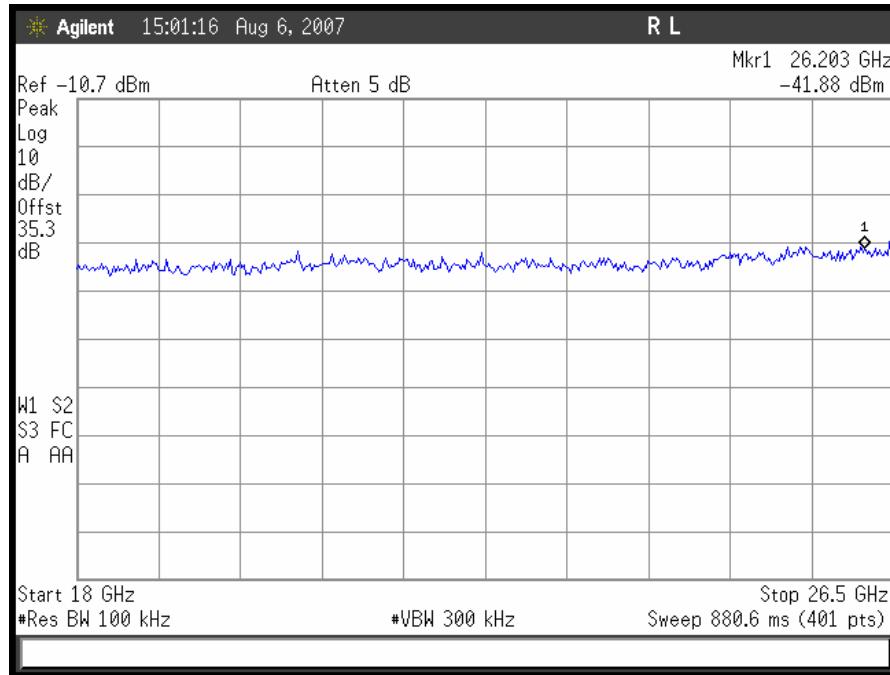
Plot 36. 802.11/a – Mid Channel Conducted Emissions 18 - 26.5GHz
