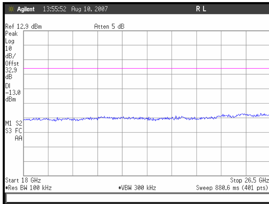
Plot 27. 802.11/g – Low Channel Conducted Emissions 18 – 26.5GHz
