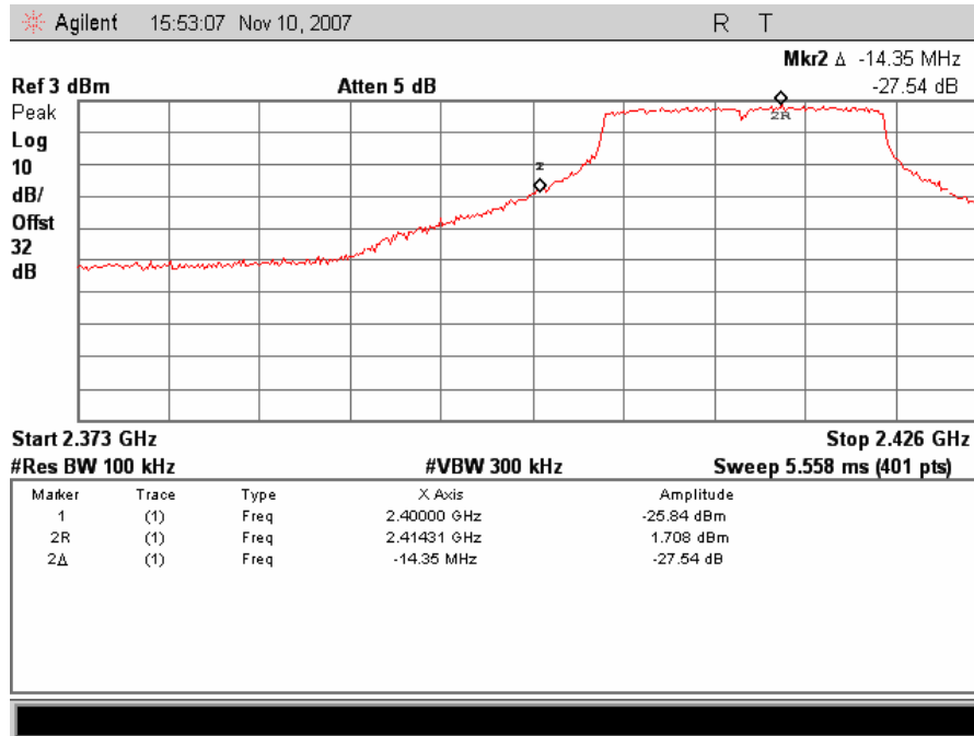
Plot 43. 802.11/g – Lower Band Edge
