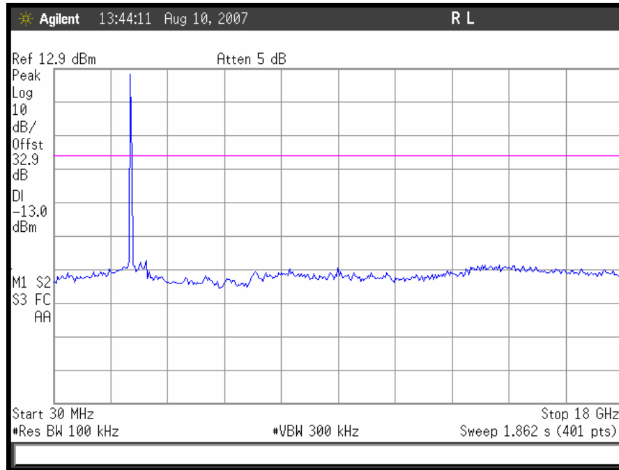
Plot 24. 802.11/b – High Channel Conducted Emissions 30MHz- 18GHz
