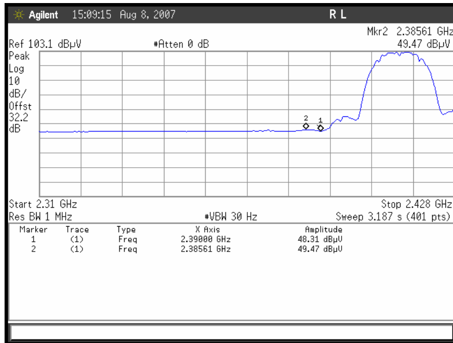
Plot 13. 802.11/b radiated restricted band 2310- 2390 MHz Avg
