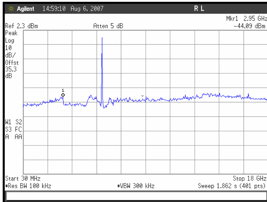
Plot 38. 802.11/a – High Channel Conducted Emissions 30MHz – 18GHz
