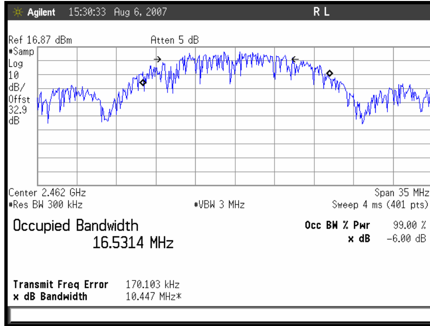
Plot 5. 802.11/b High Ch Occupied Band Width
