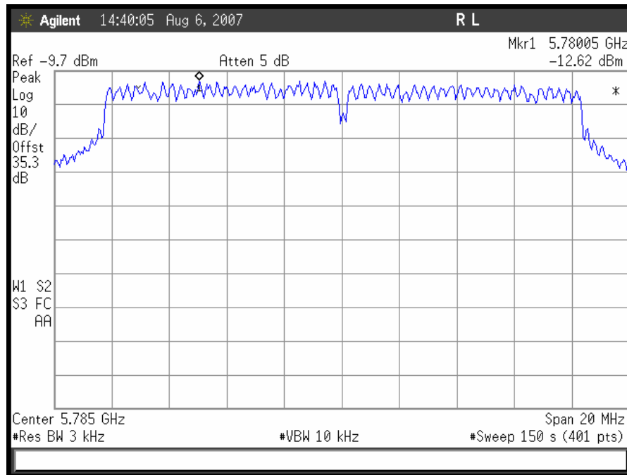
Plot 54. 802.11/a – Mid Ch Peak Power Spectral Density
