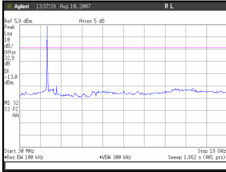
Plot 26. 802.11/g – Low Channel Conducted Emissions 30MHz - 18GHz
