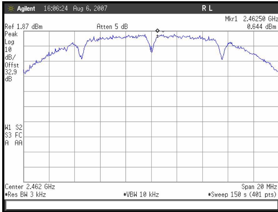
Plot 49. 802.11/b – High Ch Peak Power Spectral Density
