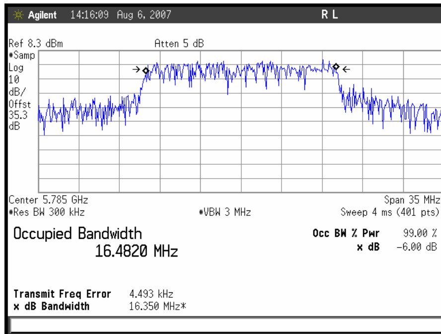
Plot 10. 802.11/a Mid Ch Occupied Band Width
