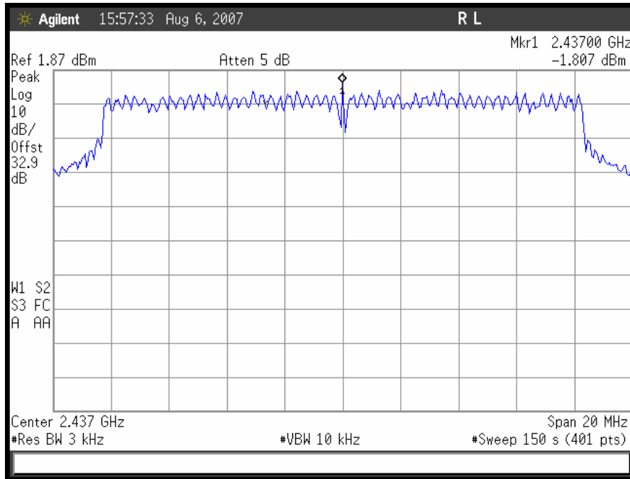
Plot 51. 802.11/g – Mid Ch Peak Power Spectral Density
