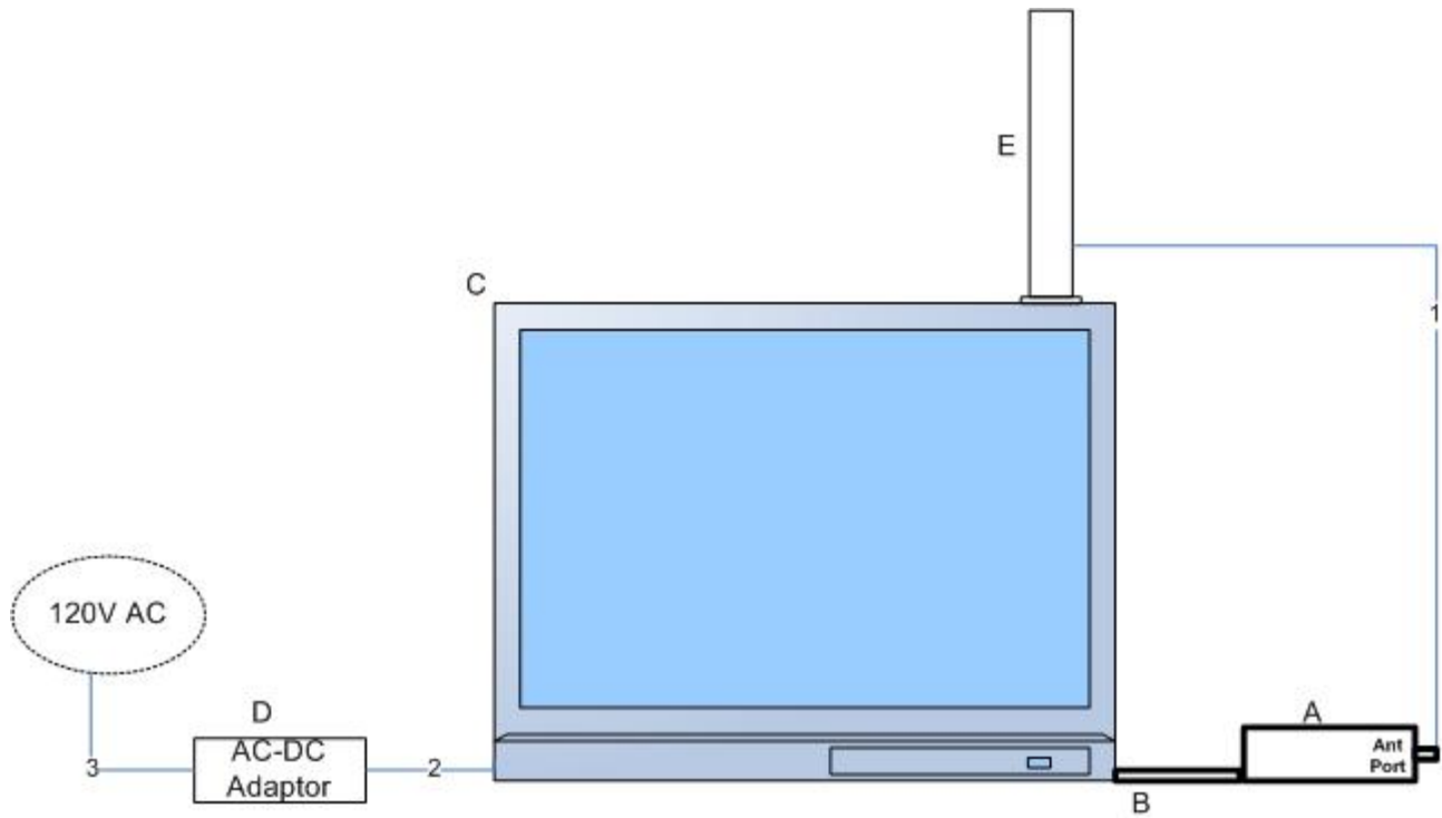
Figure 3. Block Diagram of Test Configuration (Spurious Emissions)
