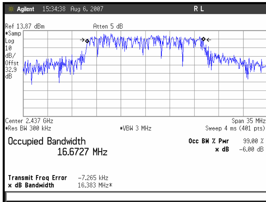
Plot 7. 802.11/g Mid Ch Occupied Band Width
