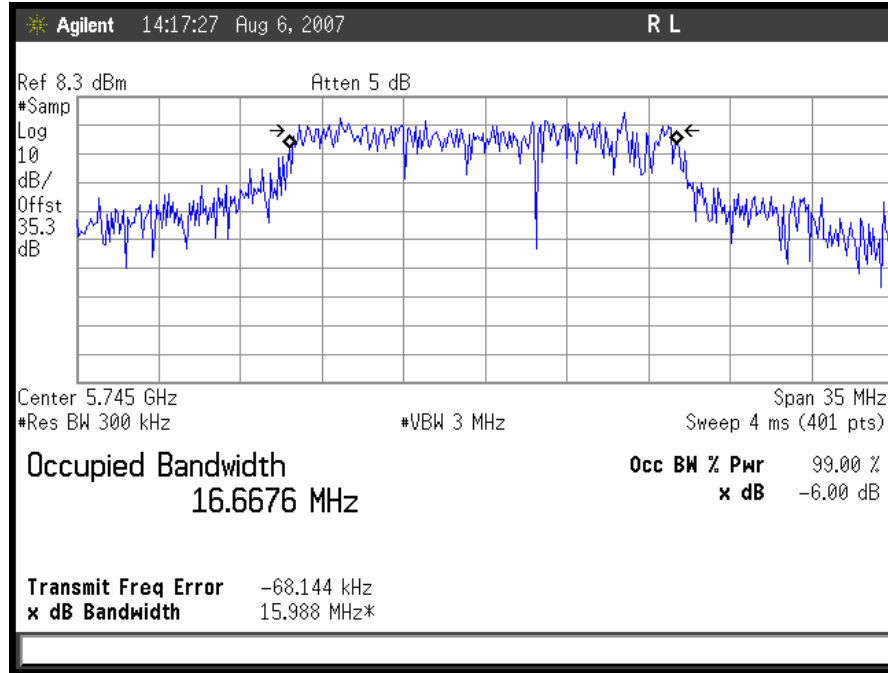
Plot 9. 802.11/a Low Ch Occupied Band Width
