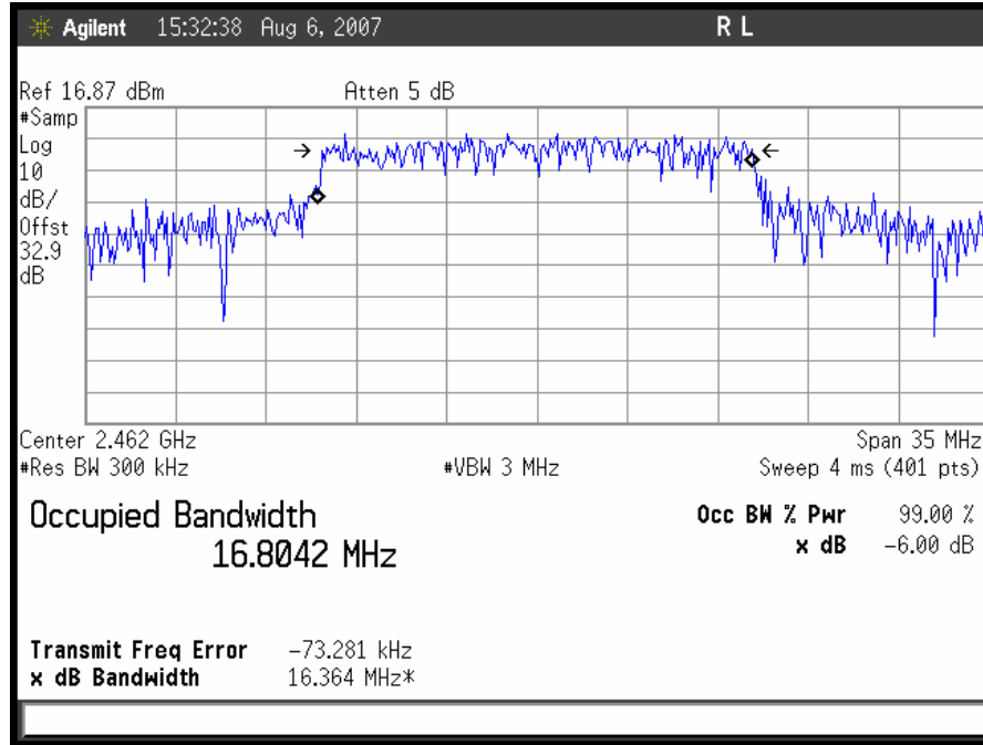
Plot 8. 802.11/g High Ch Occupied Band Width
