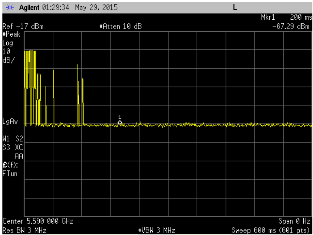
Channel Close
