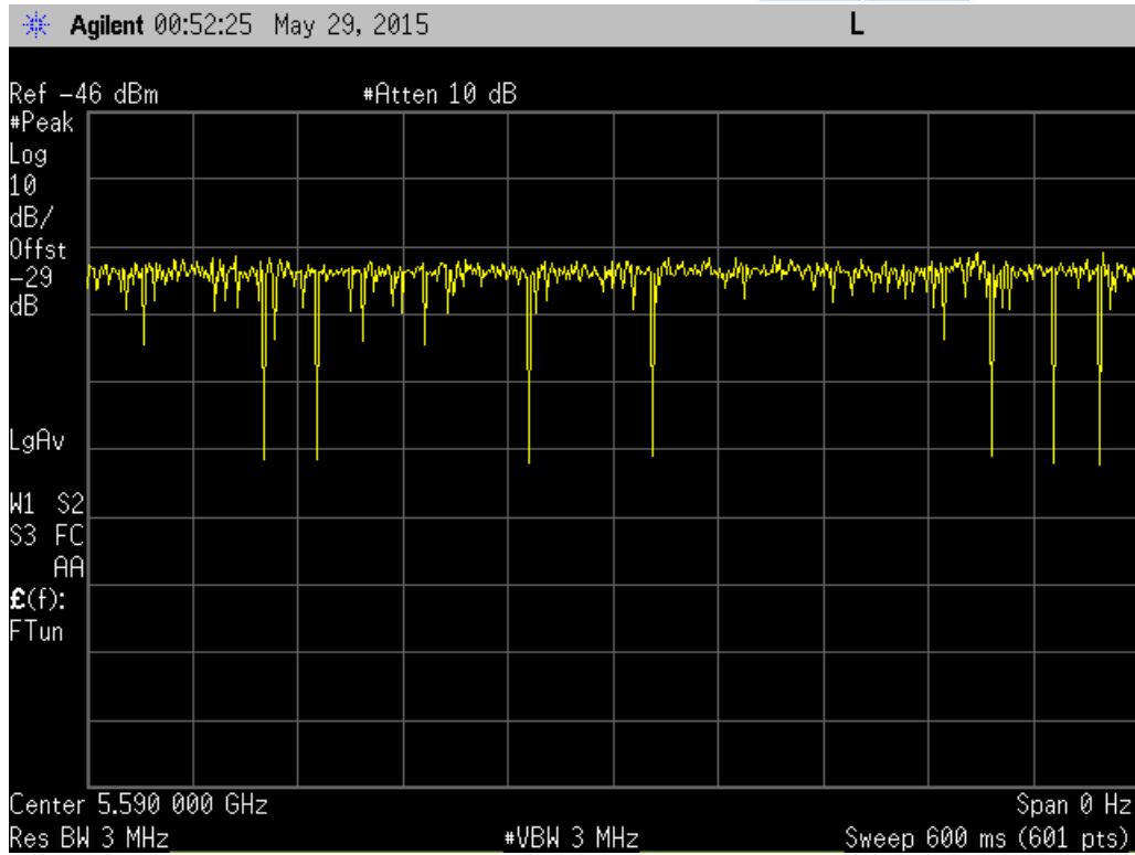
20MHz Traffic
