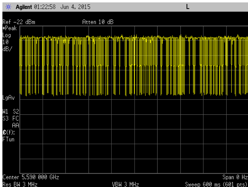
10MHz Traffic
